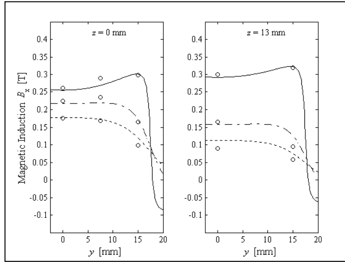
Fig. 7. Experimental comparison of the magnetic induction: analytical magnetic induction in plane x = 6 mm (–), x = 9 mm (–·–), x = 12 mm (···), (o) experimental values
