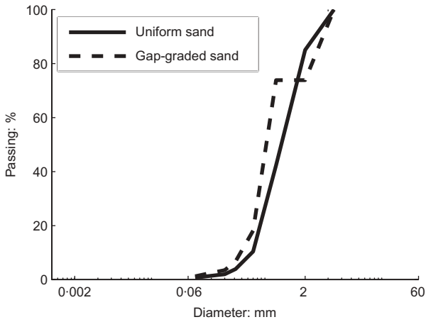
Fig. 9. Grain size distribution of uniform and gap-graded sands
