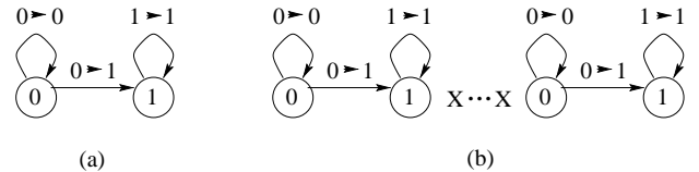
Figure 2: Scheduling automata.
