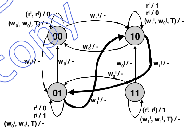
Figure 2: M_1: \langle \uparrow, 0 \rangle Idempotent Coupling Fault
