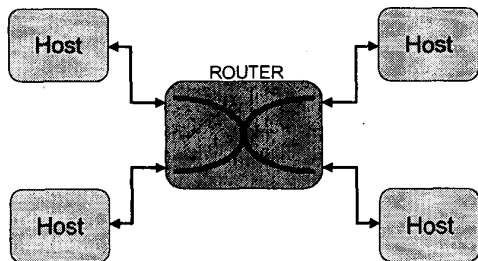
Figure 2: Network architecture
