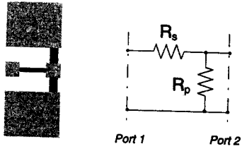
Fig. 1. Layout and schematic of the TS used for optimization.
