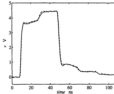
Figure 4: Output voltage waveform of the DUM driving a series connection of a 100\ \Omega resistor and an open ended 1.5 m long RG58 coaxial cable ( Z_0 = 50\ \Omega ). Dashed line: measured reference response; solid line: response of the 2-piece RBF model.
