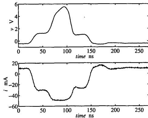
Figure 3: Measured steady state identification signals v(t) and i(t) for submodel f_1 .
