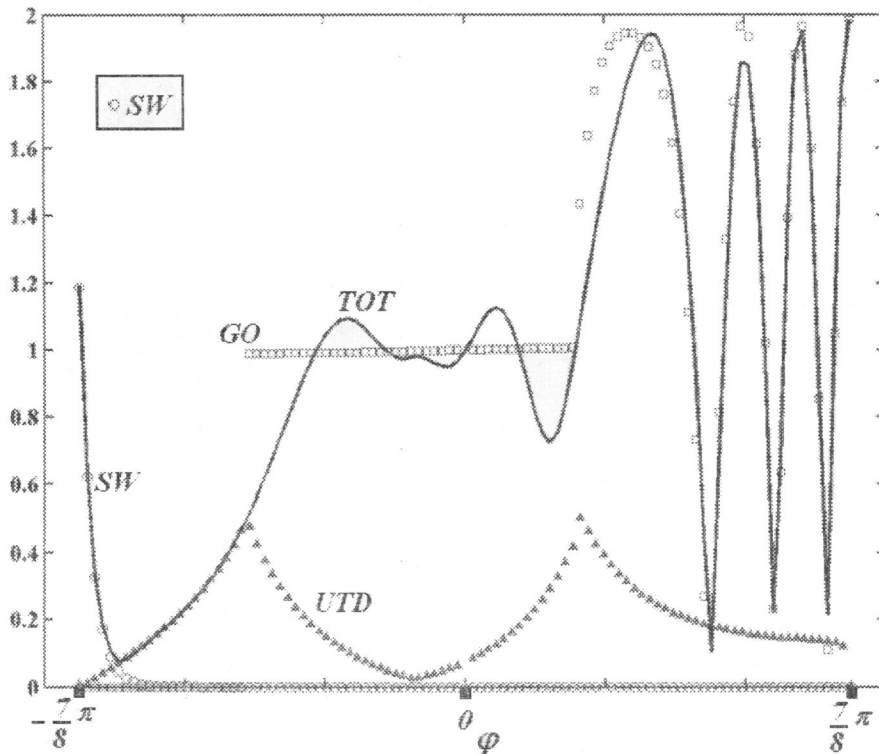
Figure 4: Total field, GO field component, UTD field component and SW field component for k\rho = 10 , \varphi_0 = \pi/2 , E_o = 0 , H_o = 1 , \Phi = 7\pi/8 , z_a = 0.01 , z_b = \sin(\theta_b) , \theta_b = 0.01 + j .
