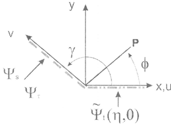
Figure 2: Domain definition for \tilde{\psi}_t(\eta, 0) , \psi_s(v) and \psi_\tau(v, \gamma) .
