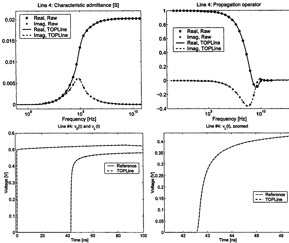
Figure 2: Line 4: Rational approximation of characteristic admittance (top left) and propagation operator (top right). Near and far terminations voltages (bottom panels).
