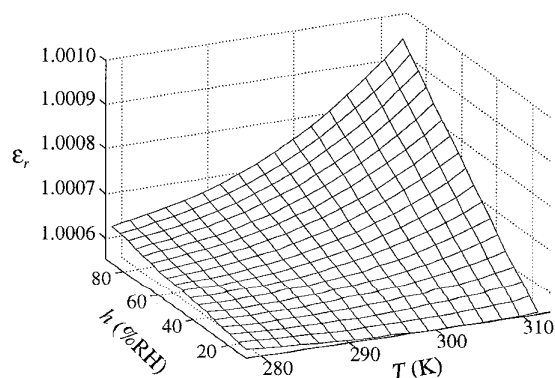
Fig. 1. Theoretical behaviour of air relative permittivity.
