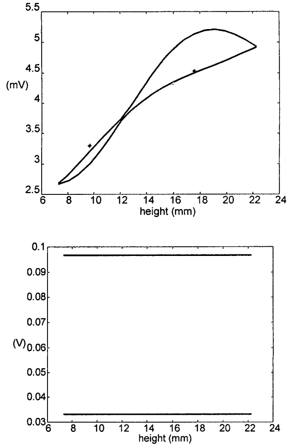
Figure 5. Test of Kriging predictions: the top panel refers to the mean crosstalk at 101 kHz, and the bottom panel refers to the maximum crosstalk over the 100-500 MHz band. In each panel the band between the two curves represents the interval mean voltage +/- standard deviation vs. height above ground, for fixed fractal dimension ( D=1.29 ). The "*" represents the exact value at test points.
