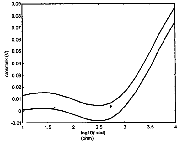
Figure 10. Test of Kriging results of the 3-dimensional experiment design. The band between the two curves represents the interval mean voltage +/- one standard deviation. The symbol "**" represents the test points.
