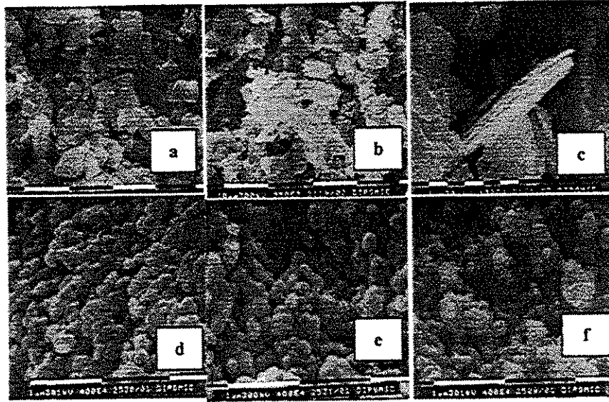
Figure 4: Crystal morphologies: a) tabular crystals ( \text{BaCl}_2 in the jet c_{A0} = 34 \text{ mol/m}^3 , \alpha = 0.1 ); b) dendritic crystals ( \text{BaCl}_2 in the jet c_{A0} = 34 \text{ mol/m}^3 , \alpha = 1.0 ); c) particular of a dendritic crystal in (b) conditions; d) round-shaped crystals ( \text{BaCl}_2 in the jet c_{A0} = 34 \text{ mol/m}^3 , \alpha = 3.0 ); e) round-shaped crystals ( \text{Na}_2\text{SO}_4 in the jet c_{A0} = 34 \text{ mol/m}^3 , \alpha = 3.0 ); f) round-shaped crystals ( \text{BaCl}_2 in the jet c_{A0} = 341 \text{ mol/m}^3 , \alpha = 0.1 ).
