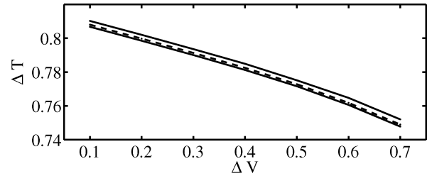
Fig. 6. Eye opening parameter values (defined in Fig. 4) for the eye diagrams of waveforms v_3 computed in test case #1. Solid thin line: reference; solid thick line: macromodels (M1 set); dashed thick line: macromodels (M2 set).
