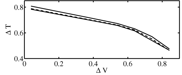
Fig. 5. Eye opening parameter values (defined in Fig. 4) for the eye diagrams of waveforms v_2 computed in test case #1. Solid thin line: reference; solid thick line: macromodels (M1 set); dashed thick line: macromodels (M2 set).
