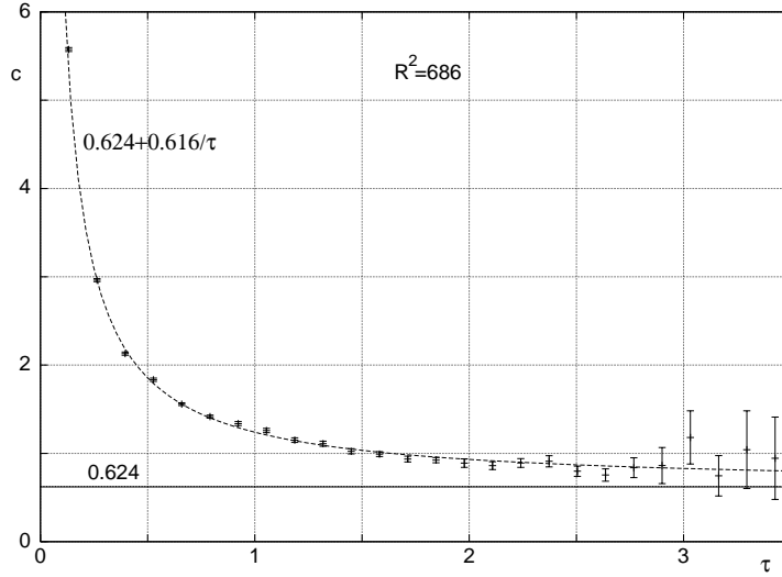
Fig. 5. The value c(\tau) for the GNS run with fixed energy ( \ell = 1, m = 0 ), R^2 = 686 . The times \tau , in the horizontal axis are given in 1/\lambda_{max} units. Data refer to a 24–real modes truncation ( 2K = 24 ) and to values of \tau to which already corresponds a linear graph of F(p; \tau) . The datum with smallest \tau has not been used in constructing of the fit (but it matches it, nevertheless).
