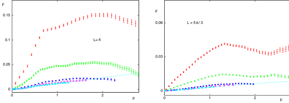
Fig. 6. Numerically computed values of F(p; V) , and corresponding error bars, for L = \pi (left) and L = 5\pi/3 (right). In each panel we have 5 curves, corresponding to T_0 \approx 0.58, 1.75, 5.27, 7.81, 10.74 (in 1/\lambda_{max} units), ordered clockwise with growing T_0 . Only three curves are clearly distinguishable because the three of highest T_0 practically overlap in their range of coexistence, which shrinks with increasing T_0 .
