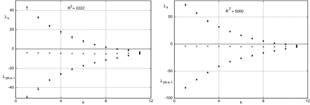
Fig. 1. Lyapunov spectra for the NS runs with normal viscosity ( \ell = 1 ) at R^2 = 2222 (left) and R^2 = 5000 (right), and corresponding GNS runs with constrained energy Q_0 . The 2K - 2 nontrivial exponents are drawn by associating each value of the abscissa k = 1, 2, \dots, K - 1 with the k -th largest exponent \lambda_k and the k -th smallest exponent \lambda'_k = \lambda_{2K-k-1} . The symbols “+” refer to the NS spectra, the “*” to the GNS spectra, and the “x” to the sums (\lambda_k + \lambda'_k)/2 for the NS case. There is no “pairing” of the exponents to a common average value, unlike the cases of isokinetic Gaussian systems [27]. Essentially identical results have been obtained by studying the ED and GED equations.
