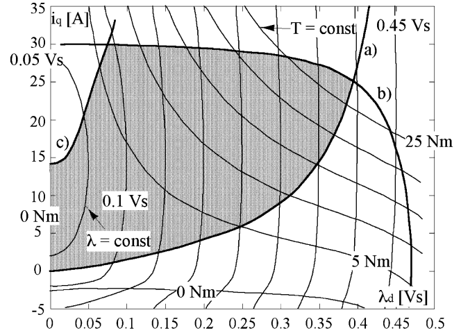
Fig. 9. Constant-torque and constant-flux loci in the (\lambda_d, i_q) plane.
