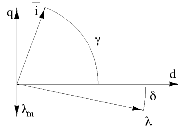
Fig. 3. Current and flux vectors.
