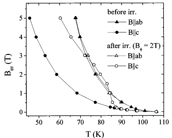
FIG. 7. Comparison of the anisotropy of IL's before and after irradiation, for the magnetic field applied parallel and perpendicular to ion tracks, i.e., to the c axis of the samples.
