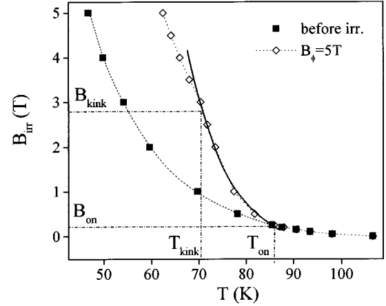
FIG. 4. Irreversibility lines for the unirradiated sample and for samples irradiated with B_{\phi} = 5 T. The solid line is a fit of the experimental data, between B_{\text{on}} and B_{\text{kink}} , with Eq. (2) (see text).
