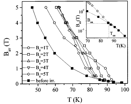
FIG. 1. Irreversibility lines for the unirradiated sample and for samples irradiated with different doses, ranging from B_\phi = 1-5\ \text{T} . In the inset the onset phase point (B_{\text{on}}, T_{\text{on}}) is indicated for the sample with B_\phi = 5\ \text{T} .
