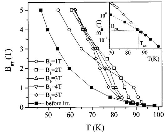
FIG. 1. Irreversibility lines for the unirradiated sample and for samples irradiated with different doses, ranging from B_\phi = 1-5\ \text{T} . In the inset the onset phase point (B_{\text{on}}, T_{\text{on}}) is indicated for the sample with B_\phi = 5\ \text{T} .
