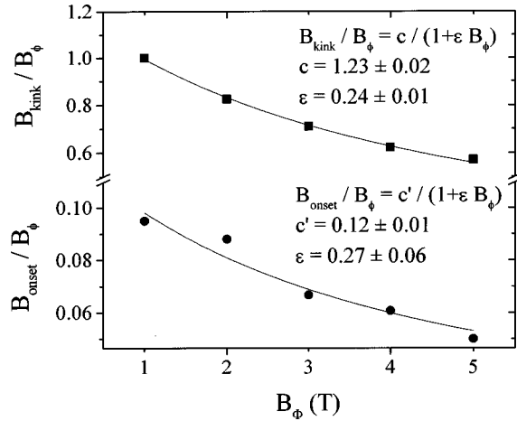
FIG. 5. Field of the kink and field of the onset, normalized to B_{\phi} , as a function of B_{\phi} . The curves are fits of the data with Eqs. (3) and (4), with the fitting parameters reported in the figure.
