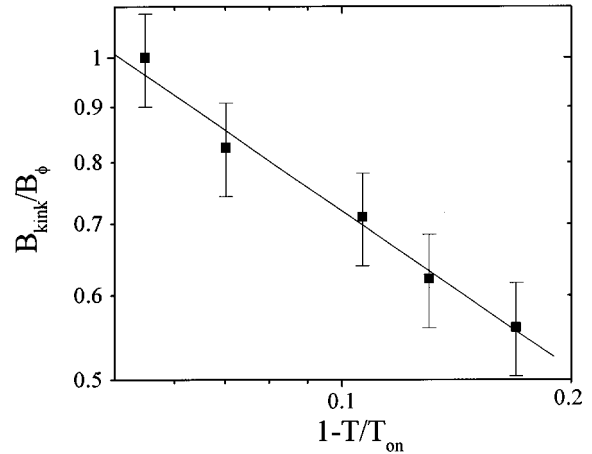
FIG. 6. B_{\text{kink}}/B_{\phi} as a function of (1 - T/T_{\text{on}}) , on logarithmic scales. The fit of data with the law B_{\text{kink}}/B_{\phi} \propto (1 - T/T_{\text{on}})^{\beta} gives the value \beta = 0.49 \pm 0.03 .
