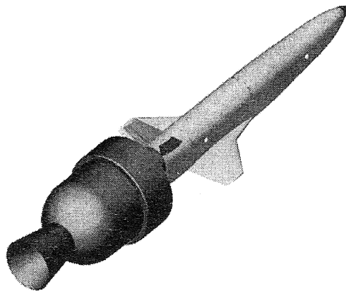
Fig. 3: Mini-FTB/A (STAR17A)
