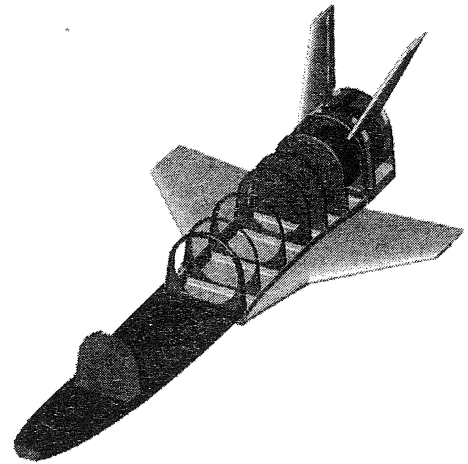
Fig. 10: Mini-FTB internal structure
