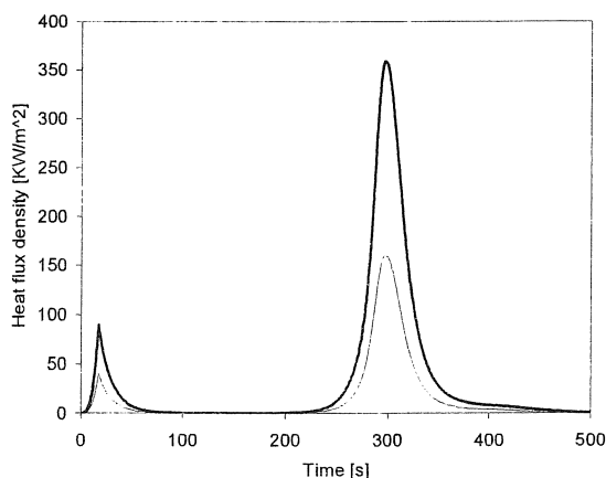
Fig. 19: heat flux density versus time for the Mini-FTB (nose radius drawn to 1:5 and 1:1 scale)
