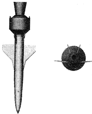
Fig. 8: upper and front view of the Mini-FTB and its propulsion system
