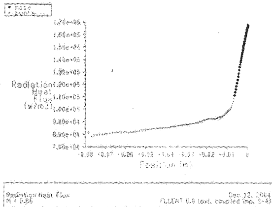
Fig. 21: variation of the heat flux along the body longitudinal axis for the demonstrator's nose (drawn to 1:1 scale) and front part
