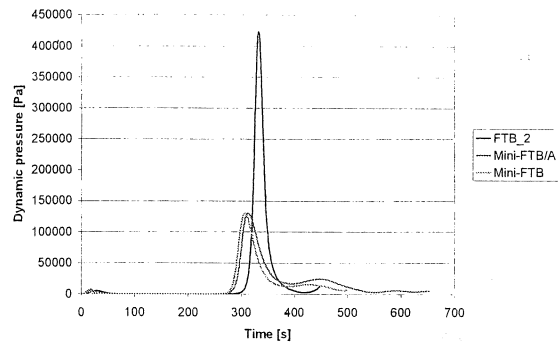
Fig. 4: dynamic pressure's values comparison
