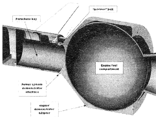
Fig. 17: recovery and power system CAD model
