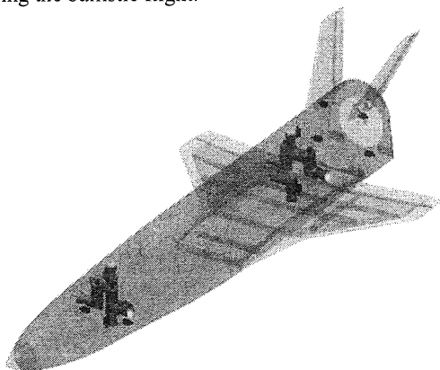
Fig. 14: internal layout of the RCS thrusters
