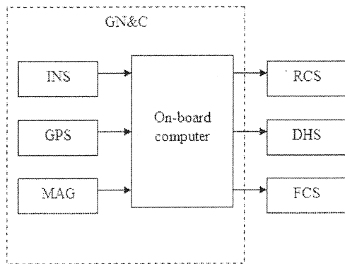
Fig. 16: GNC System architecture
