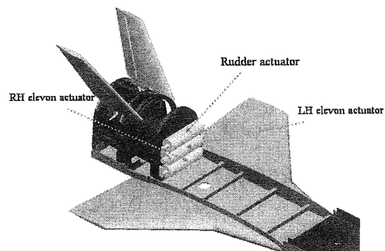
Fig. 15: Flight control system's electrical actuators
