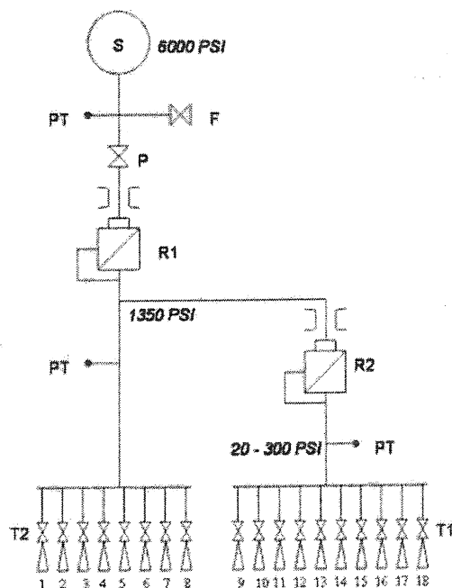
Fig. 13: RCS architecture
