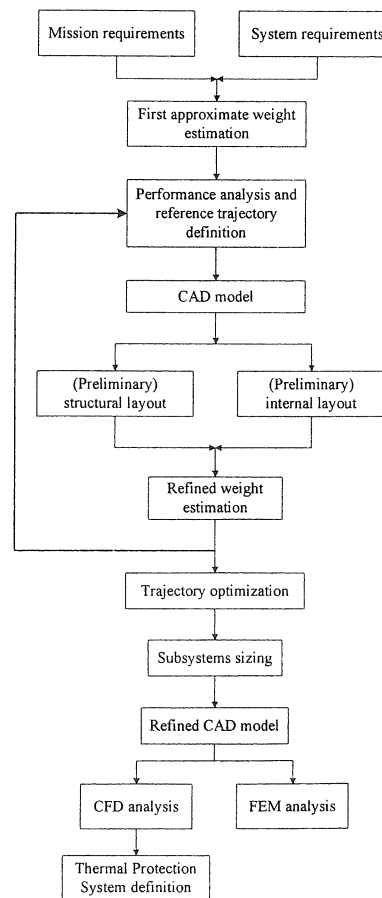
Fig. 1: design process flow chart
