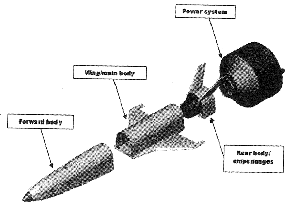
Fig. 9: Mini-FTB four main parts
