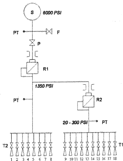
Fig. 13: RCS architecture
