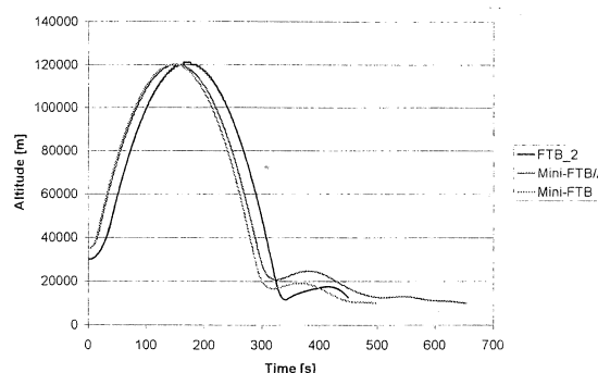
Fig. 5: trajectory comparison
