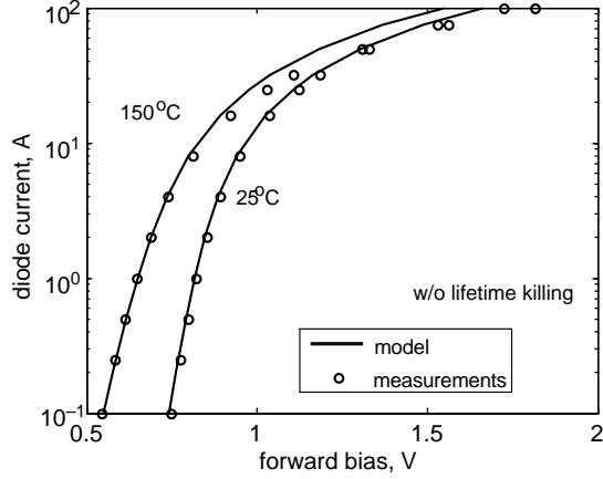
Fig. 1. Measured and simulated forward I-V characteristics for an IR PiN diode without Pt lifetime killing.
