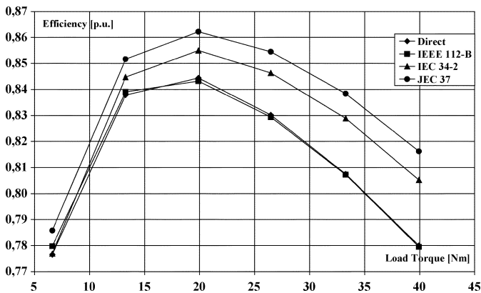
Fig. 7. Efficiency of the 4-kW motor.
