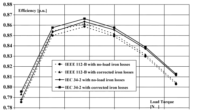
Fig. 15. Efficiency variation due to temperature corrections of the iron losses for the 15-kW motor.
