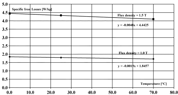
Fig. 13. Specific iron losses versus temperature with flux densities of 1.0 and 1.5 T.
