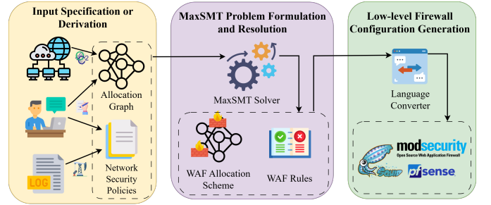
Fig. 1: The workflow of the proposed approach
