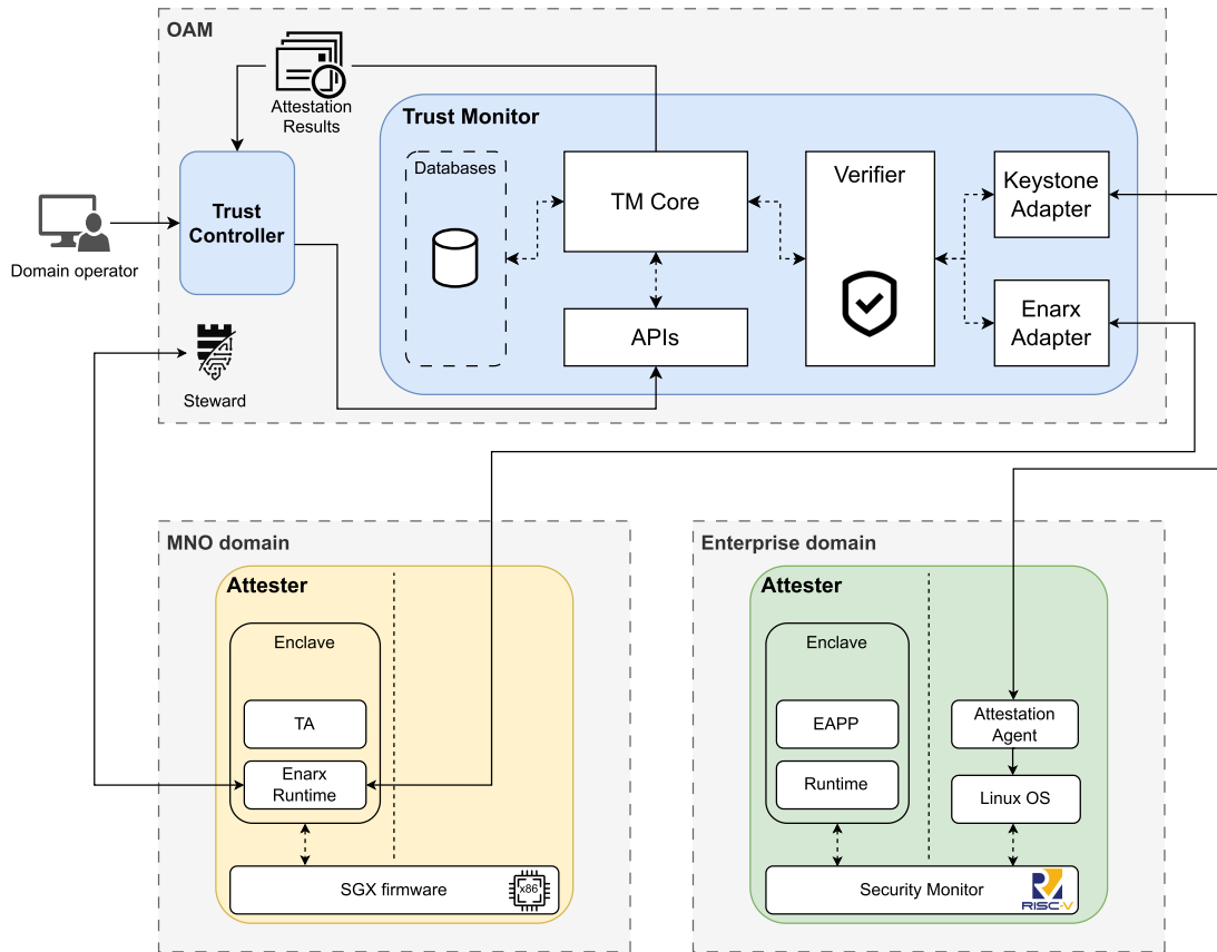
FIGURE 9. Attestation of trusted applications in the TNED.
