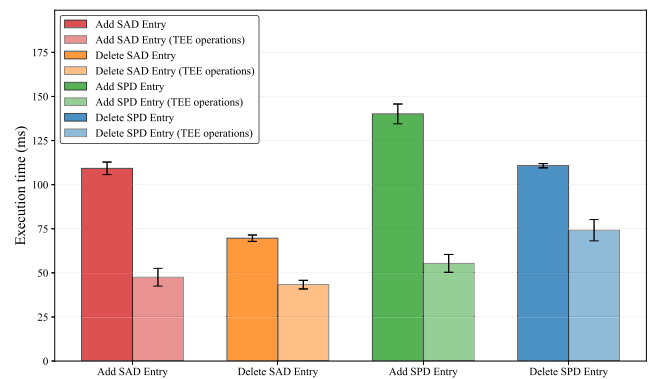
FIGURE 11. Overall and trusted operations in Keystone.
