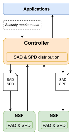
FIGURE 4. I2NSF IKE-less architecture.
