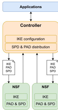
FIGURE 3. I2NSF IKE architecture.
