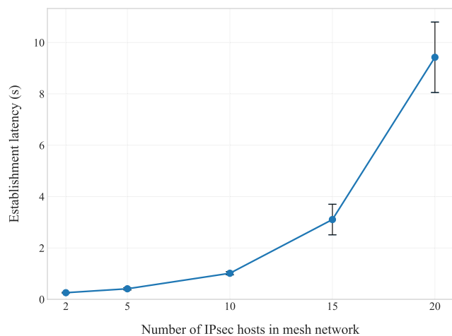
FIGURE 13. End-to-end establishment latency based on the number of concurrent tunnels.
