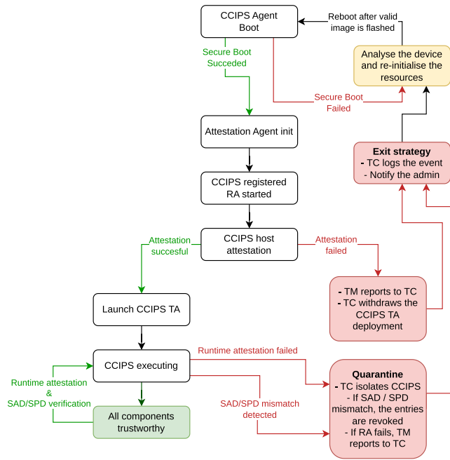
FIGURE 8. TNED verification lifecycle.
