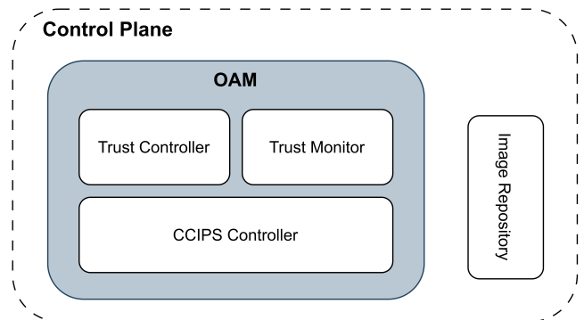
FIGURE 2. TNED control plane.
