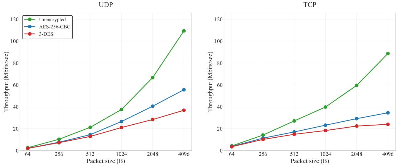
FIGURE 14. TCP and UDP throughput comparison across different packet sizes.
