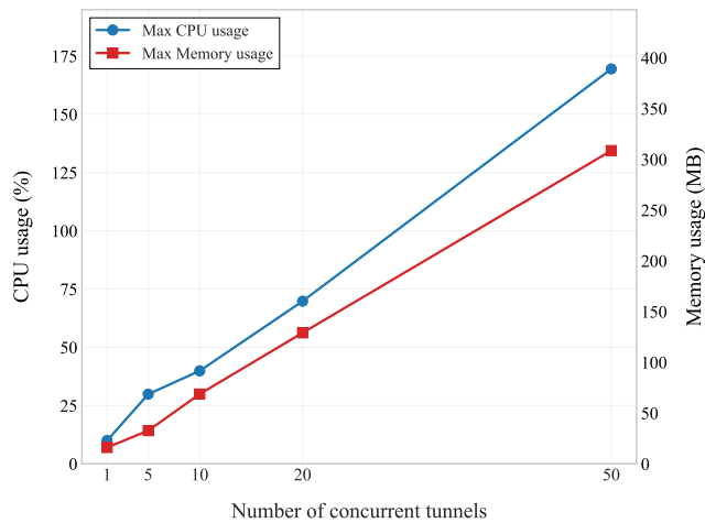
FIGURE 16. Maximum CPU and memory usage of the CCIPS Controller while establishing a different number of concurrent IPsec tunnels.
