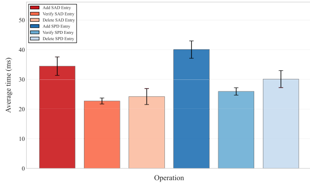
FIGURE 12. Operations performed in Enarx.
