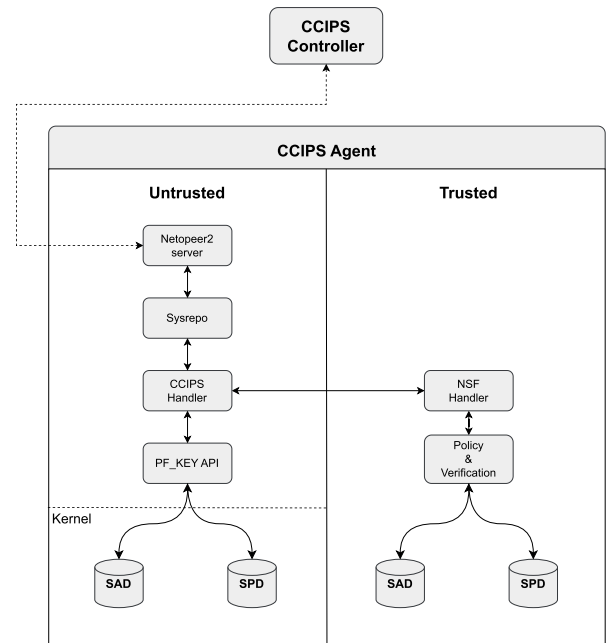
FIGURE 5. CCIPS agent architecture.
