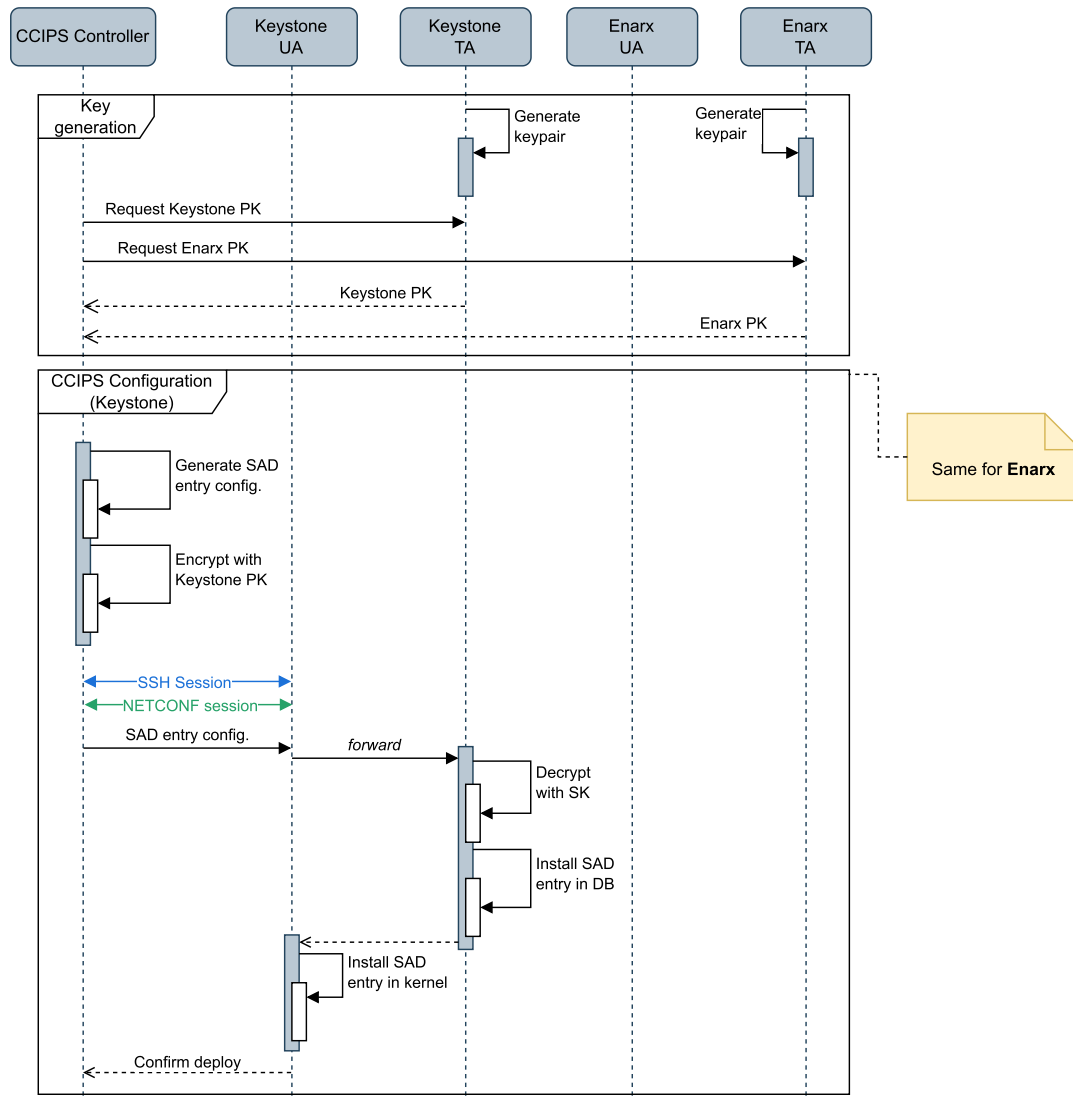
FIGURE 6. SAD configuration process.
