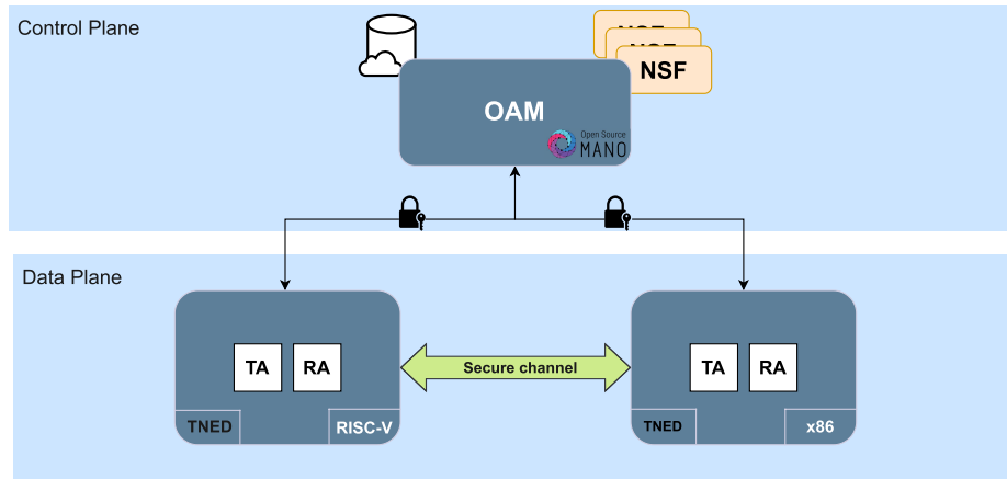
FIGURE 1. TNED architecture.
