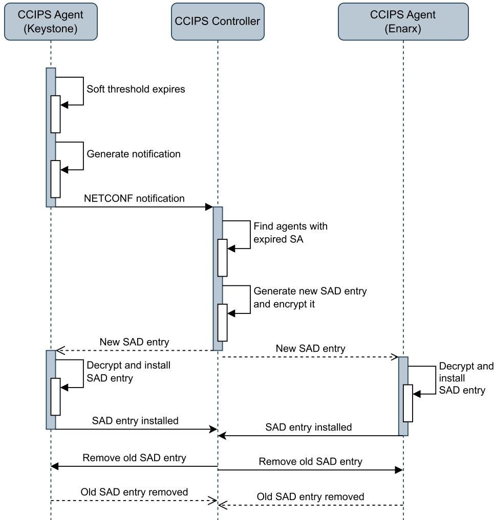
FIGURE 7. Re-keying process.
