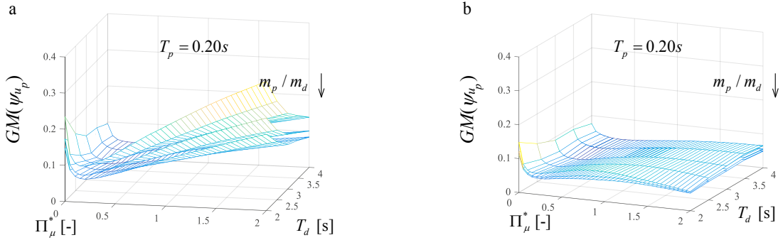
Fig. 3. Median value of the maximum normalized pier displacement as function of T_d and \Pi_\mu^* , for m_p/m_d=0.1, 0.15, 0.3 and T_p=0.2 s: (a) single-column bent viaduct; (b) multi span continuous deck bridge.
