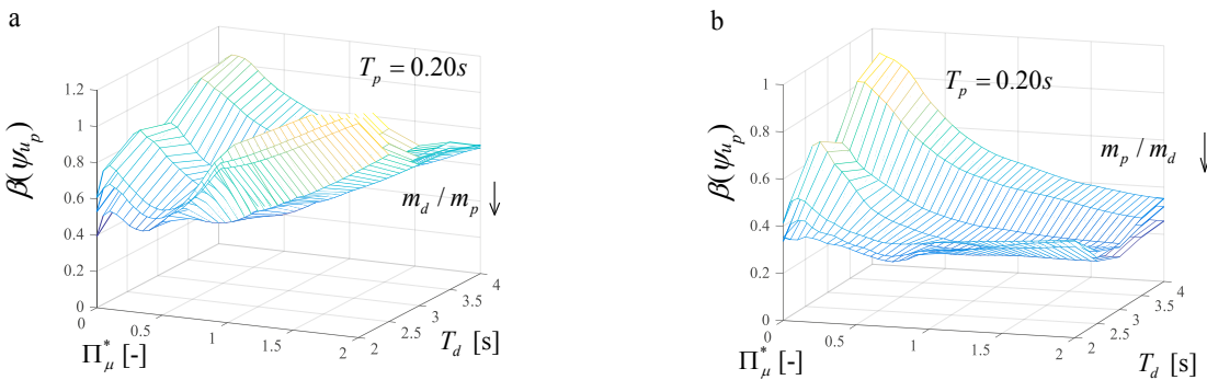
Fig. 5. Dispersion of the maximum normalized pier displacement as function of T_d and \Pi_\mu^* , for m_p/m_d=0.1, 0.15, 0.3 and T_p=0.2 s: (a) single-column bent viaduct; (b) multi span continuous deck bridge.
