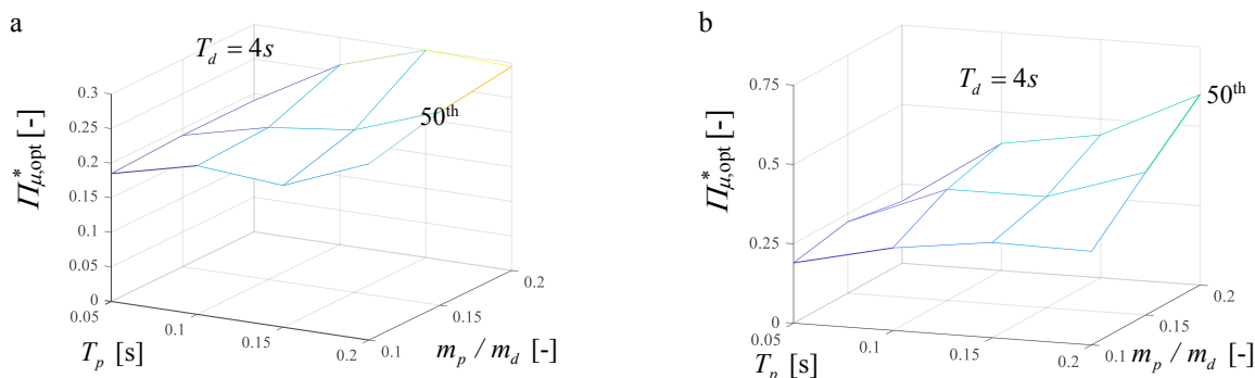
Fig. 7. Optimal friction coefficient as function of T_p , m_p/m_d and for T_d=4s : (a) single-column bent viaduct; (b) multi span continuous deck bridge.
