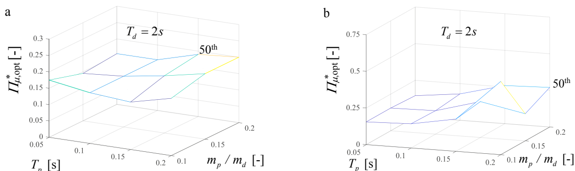
Fig. 6. Optimal friction coefficient as function of T_p , m_p/m_d and for T_d=2s : (a) single-column bent viaduct; (b) multi span continuous deck bridge.
