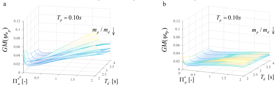
Fig. 2. Median value of the maximum normalized pier displacement as function of T_d and \Pi_\mu^* , for m_p/m_d=0.1,0.15,0.3 and T_p=0.1s : (a) single-column bent viaduct; (b) multi-span continuous deck bridge.
