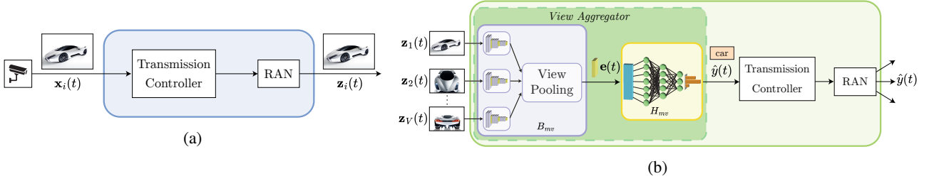
Figure 7: Schematic representation of the operations performed by a source node (a) and the central controller (b) in the non-selective centralized inference scheme (CI).
