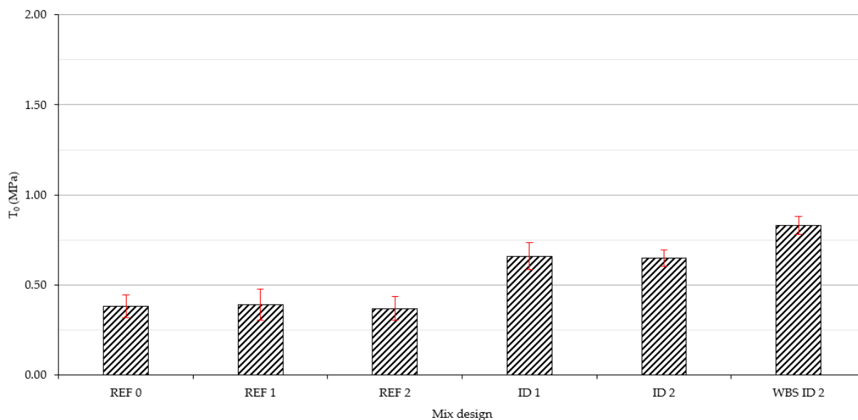
Figure 8. T_0 results after 28 days of curing, with standard deviation shown in red.
