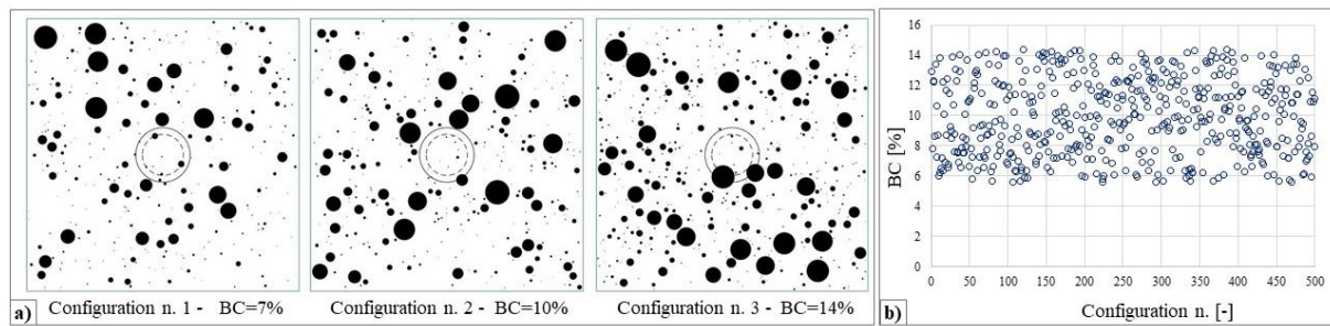
Figure 4. a) Three of the 500 configurations generated as output by the PBE code, vers.1.3. Different block sizes and positions are shown, as well as different BC values; b) BC of the n=500 configurations generated.
