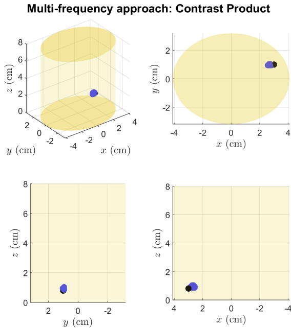
Figure 4. Multi-frequency projections with the contrast product method, obtained over the 6 – 11 GHz range, considering the multi-position configuration, with the contaminant located in L_2 = (3, 1, 0.8) cm.
