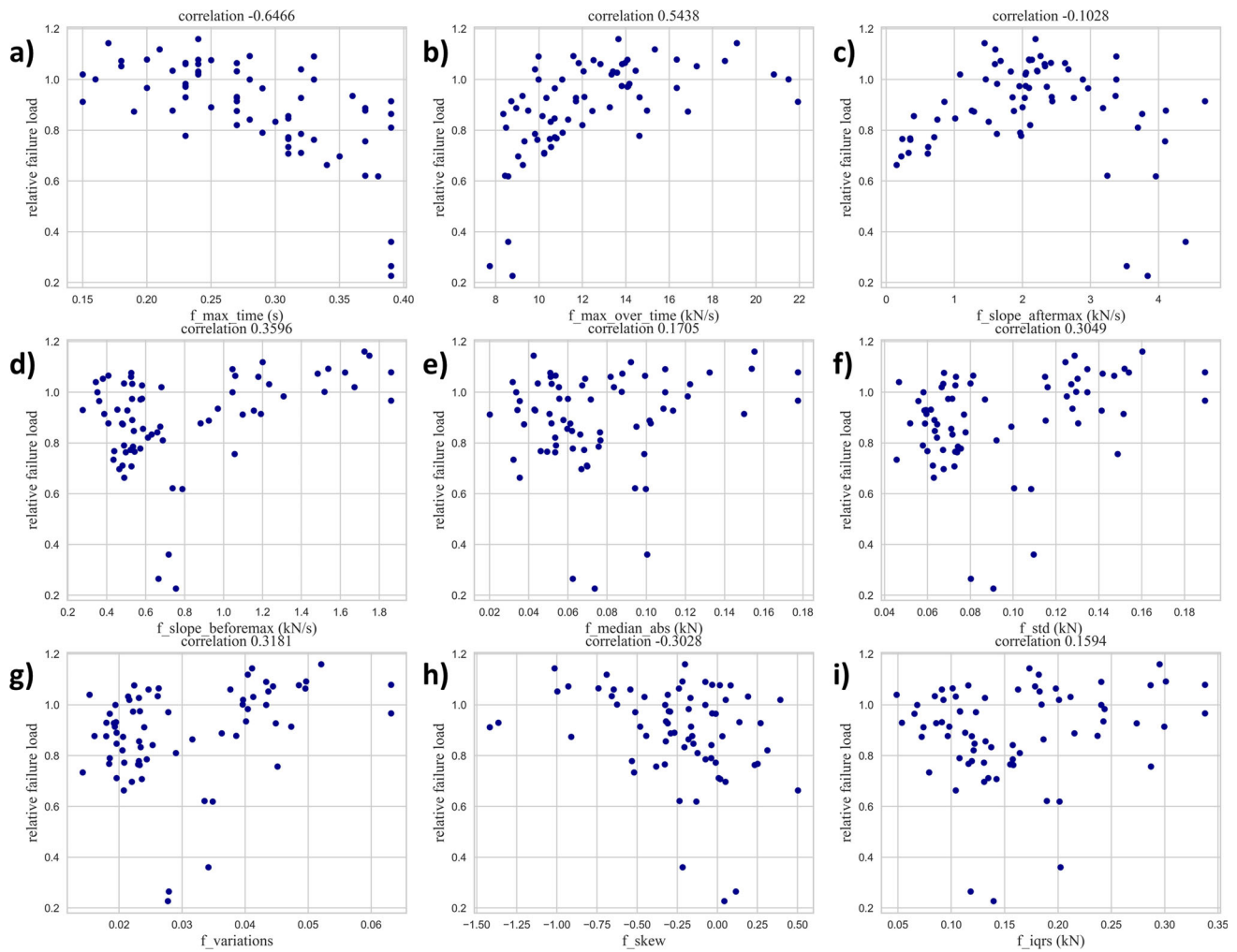
Fig. 12 Scatter plots and correlation coefficients of the features extracted from the electrode force signals; the plots represented from a) to i) refer to the features defined from Eq. (12) to Eq. (20)
