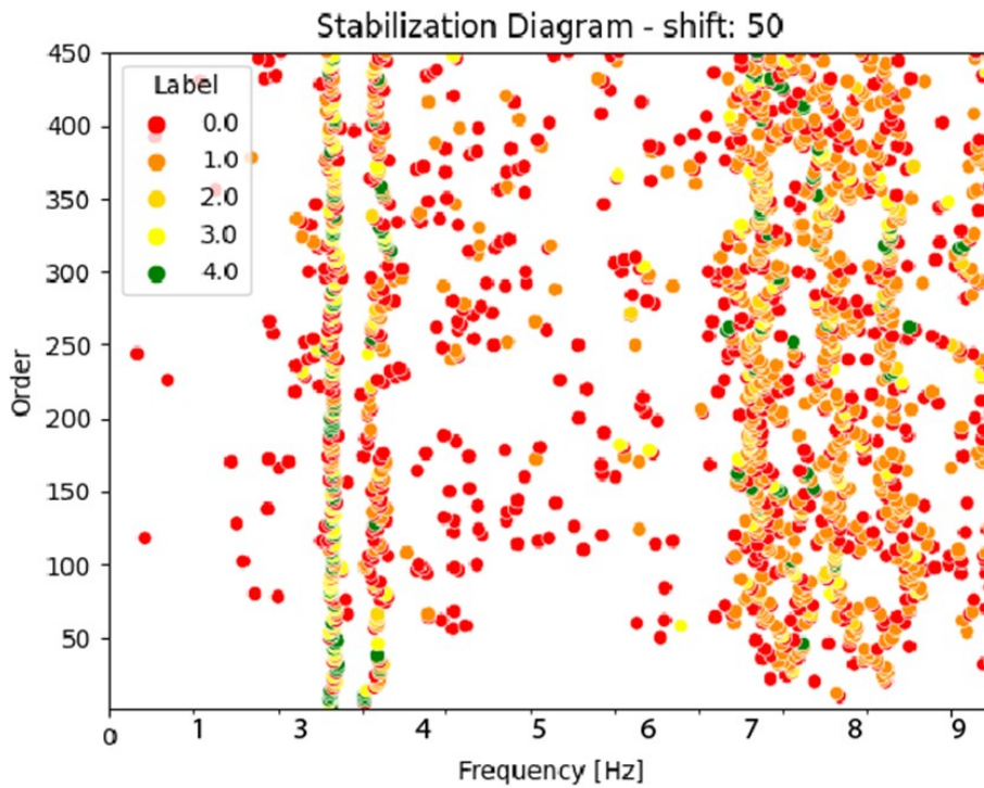
Figure 6 – Example of stabilization diagram
