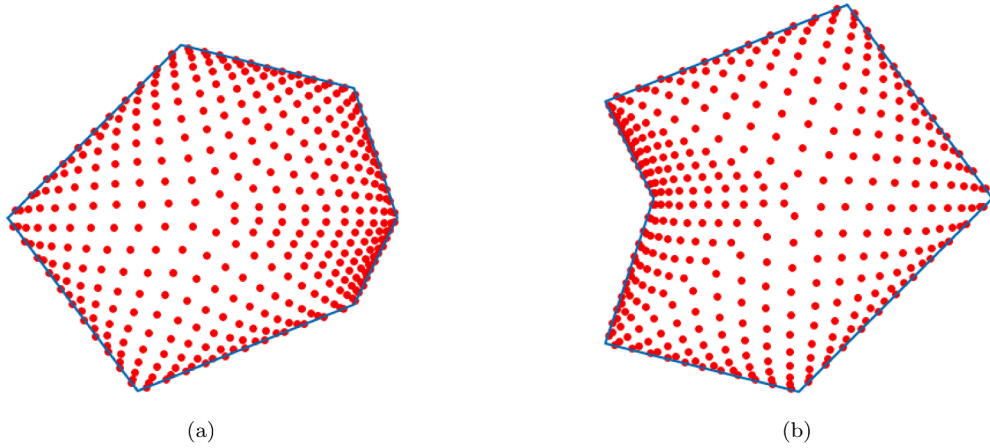
Fig. 5. Points distribution generated by using the Algorithm 1 on general polygons.
