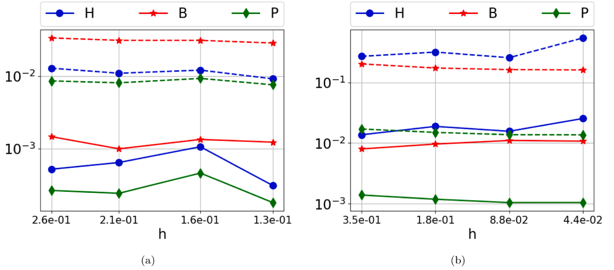
Fig. 8. Tests 1, 2, and 3: Behaviour of the metrics (35) and (36) computed on the test datasets for each method and for each test mesh refinement. Left: Voronoi. Right: Convex-Concave.
