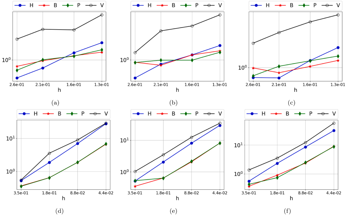
Fig. 14. Test 3: Time required (in seconds) to assemble the global system matrix and solve the discrete problem associated with (53). Each column refers to a value of \lambda , namely 1.0, 0.5, and 0.1 from left to right. First row: Voronoi. Second row: Convex-Concave.
