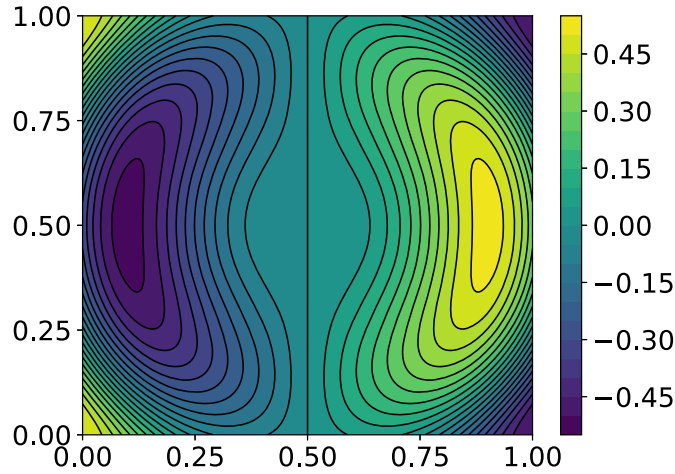
Fig. 9. Test 2: Contour plot of the exact solution u defined in (50).
