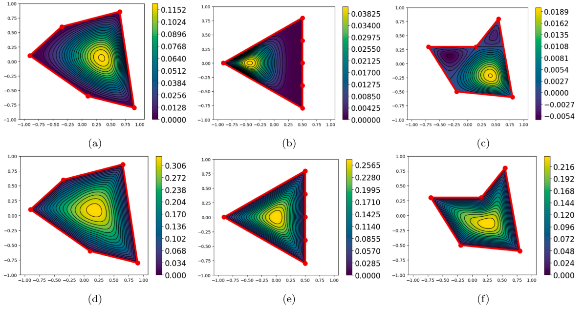
Fig. 2. Different alternatives to define the bubble function \psi_E^0 for a convex polygon (left), a triangle with hanging nodes (center), and a concave polygon (right). The top row refers to definition (21), whereas the bottom row refers to definition (23).
