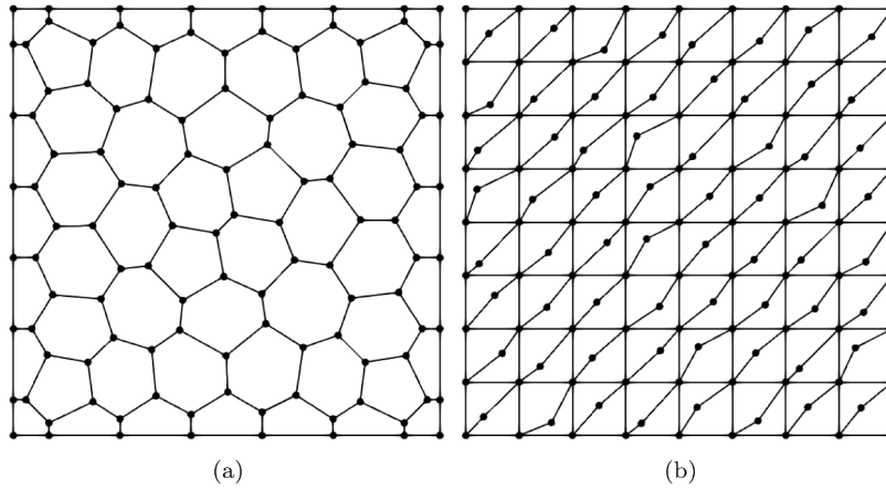
Fig. 4. Tests 1, 2, and 3: Second mesh in the two considered families of meshes used in the test phase. Left: Voronoi. Right: Convex-Concave.
