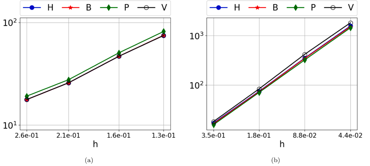
Fig. 11. Test 2: Condition number of the global system matrix associated with Problem (49). Left: Voronoi. Right: Convex-Concave.
