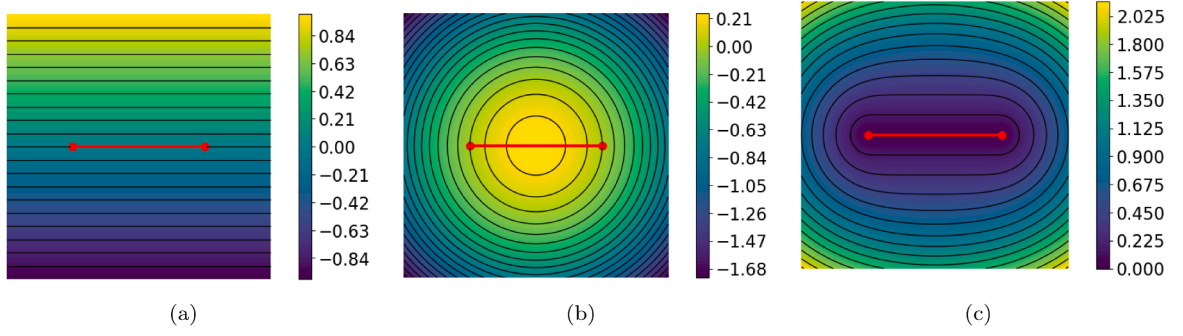
Fig. 1. Left: Distance function (20) to the line lying on the segment of extrema (-0.5, 0.0) and (0.5, 0.0) . Center: trimming function defined in (22) related the edge of extrema (-0.5, 0.0) and (0.5, 0.0) . Right: the ADF defined in (23) associated with the edge of extrema (-0.5, 0.0) and (0.5, 0.0) .
