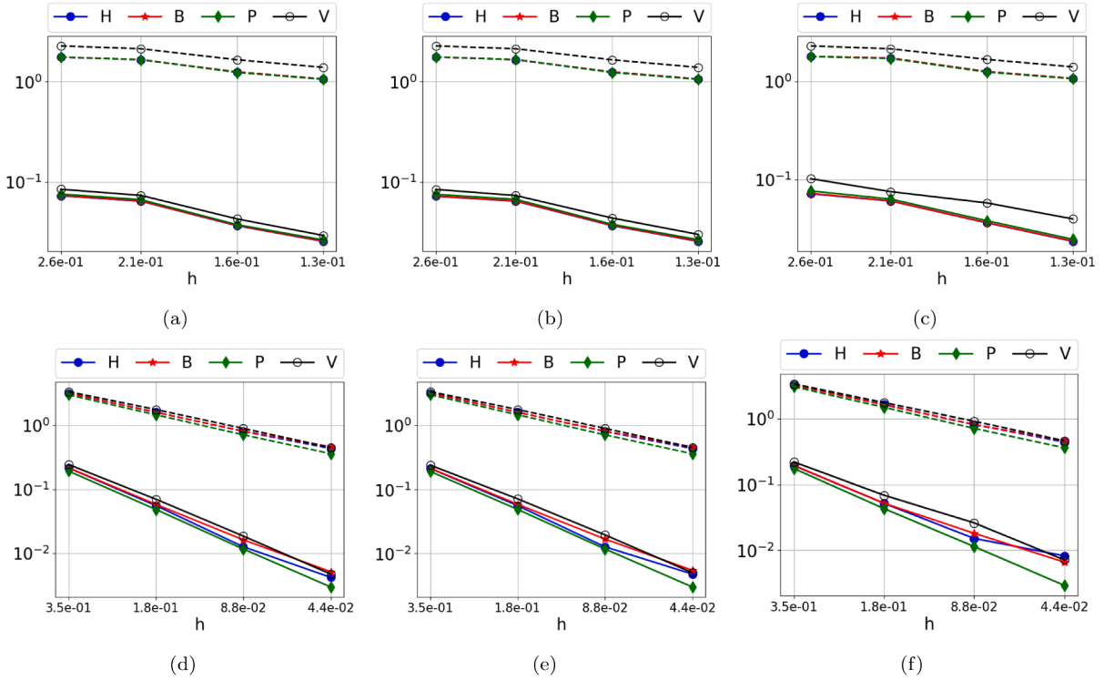
Fig. 13. Test 3: Behaviour of the errors (51) for the neural-based methods and of errors (52) for the VEM method as h decreases. Solid lines represent \text{err}_0 , whereas dashed lines denote \text{err}_V . Each column refers to a value of \lambda , namely 1.0, 0.5, and 0.1 from left to right. First row: Voronoi. Second row: Convex-Concave.
