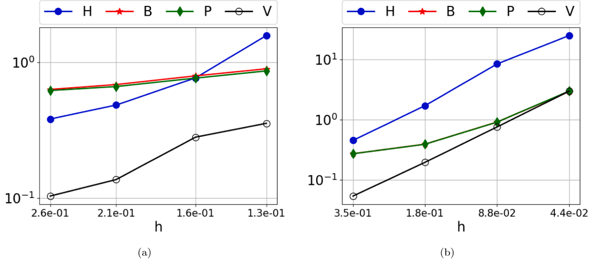
Fig. 12. Test 2: Time required (in seconds) to assemble the global system matrix and solve the discrete problem associated with (49). Left: Voronoi. Right: Convex-Concave.
