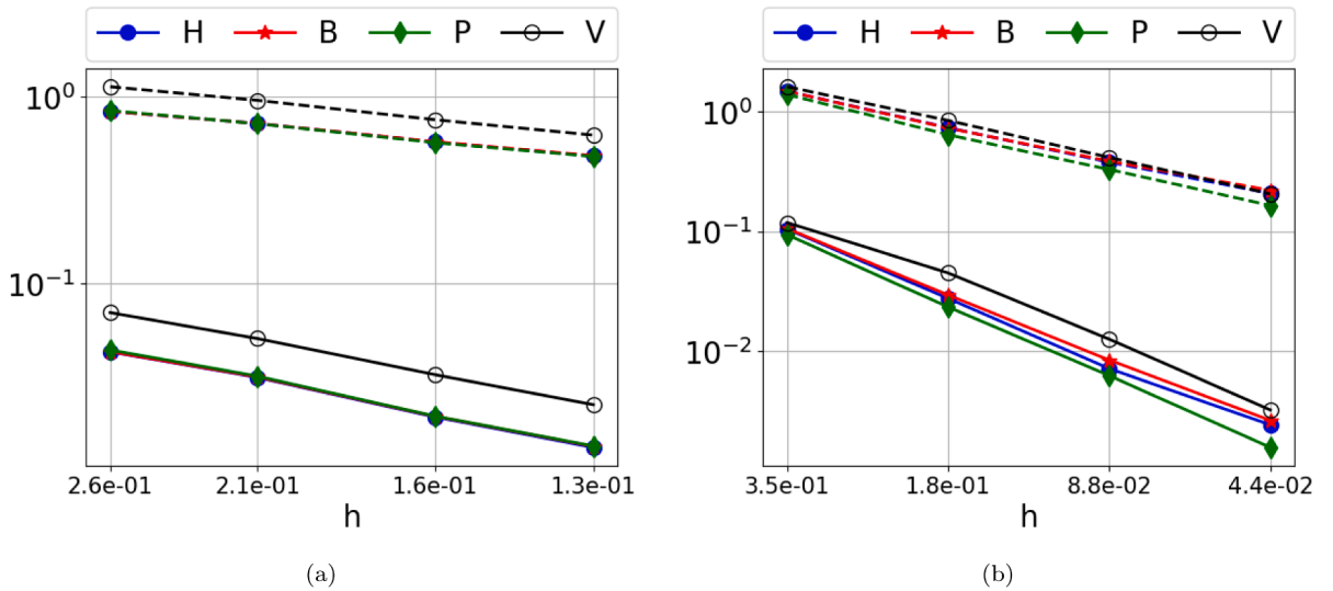
Fig. 10. Test 2: Behaviour of the errors (51) for the neural-based methods and of errors (52) for the VEM method as h decreases. Solid lines represent error err_0 , whereas dashed lines denote err_\gamma errors. Left: Voronoi. Right: Convex-Concave.
