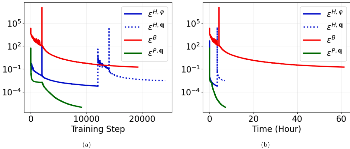
Fig. 6. Test 1: Behaviour of loss values as the number of training steps increases (left) and time increases (right) during the training phase. Dataset consisting of 1000 convex quadrilaterals.
