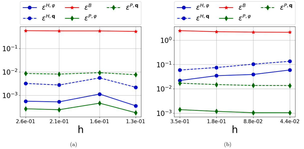
Fig. 7. Tests 1, 2, and 3: Test Loss values on each mesh refinement. Left: Voronoi. Right: Convex-Concave.
