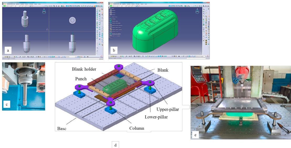
Fig. 1. - CAD design (a) of the punch and (b) of the epoxy full die matrix (800x980 mm 2 , h=100 mm); (c) the punch inserted in the milling machine; (d) the schematic representation of the full set-up; (e) photograph of the test-rig used.
