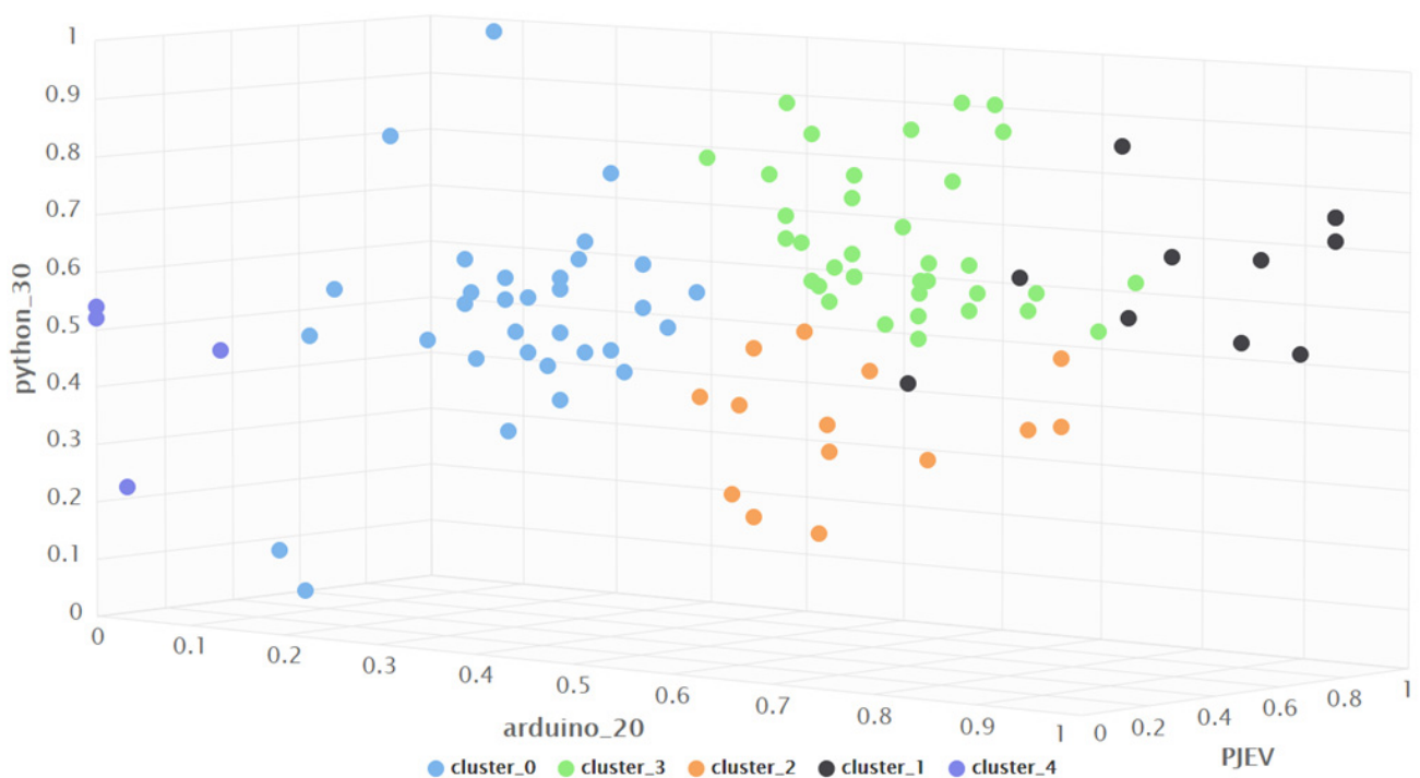
Figure 8. Cluster visualization.
