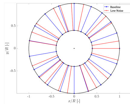
Figure 3: Baseline and low-noise stator-vane azimuthal distributions.
