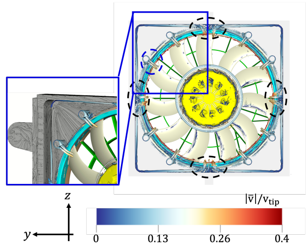
Figure 11: Mean \Lambda_2 = -2.5 \cdot 10^5 1/s iso-surfaces coloured with velocity magnitude in the upstream casing for the baseline configurations.
