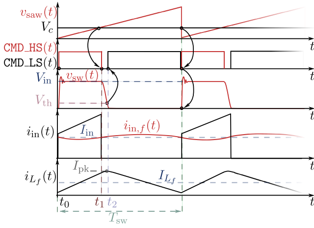
FIGURE 2 | Main voltage and current waveforms in QSW-ZVS operation of the converter in Figure 1.
