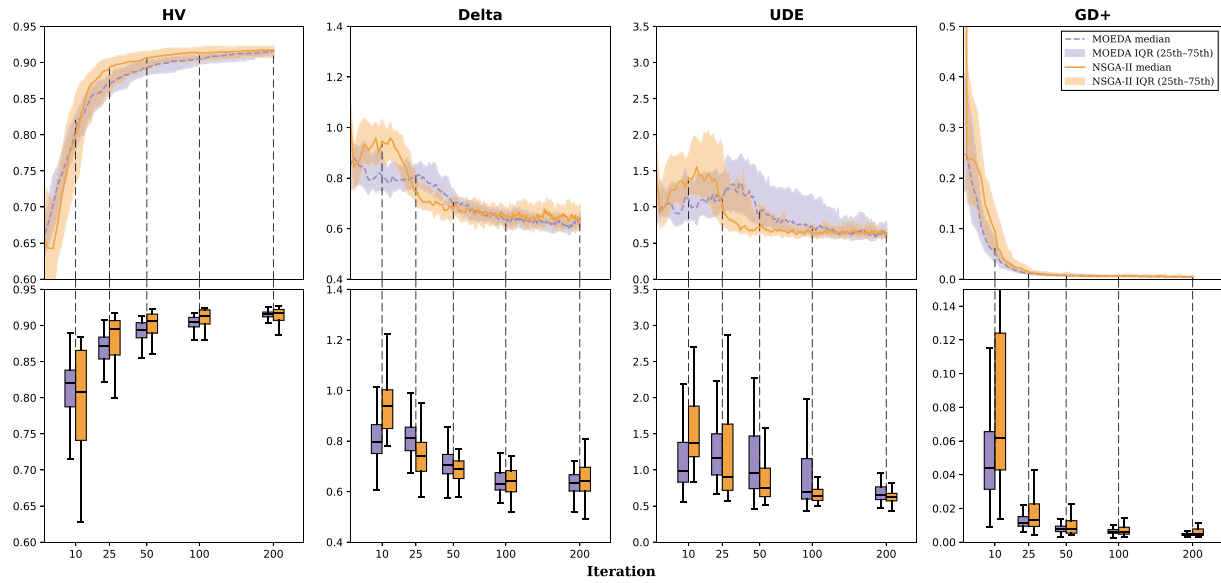
Fig. 6. Welded Beam: MOEDA-GMM champion vs NSGA-II.
