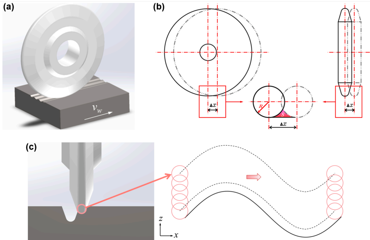
Fig. 9. Schematic diagrams of generative method((a) The generative form (b) The unground areas produced by the two methods (c) single-trajectory full-depth grinding method).
