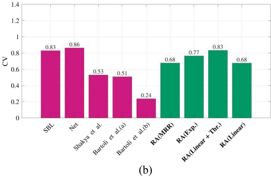
Fig. 20 Training dataset B (geometric and mechanical parameters): (a) mean prediction error for different candidate models (grey) and different RA weighting strategies (orange); (b) coefficient of variation for different candidate models (magenta) and different RA weighting strategies (green)
