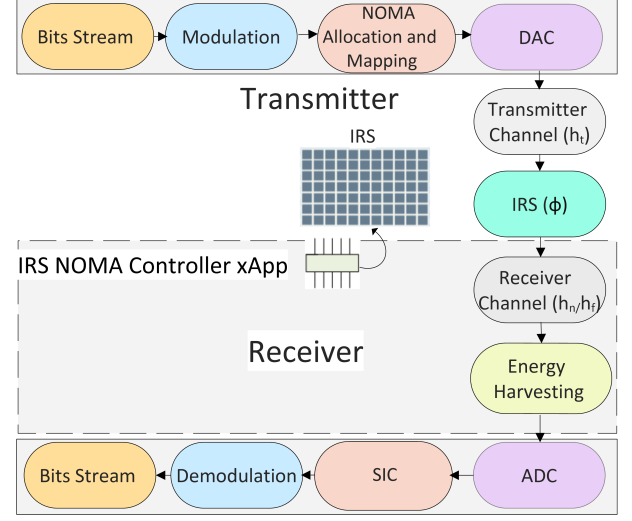
Figure 3. Diagram of an IRS-NOMA system.
