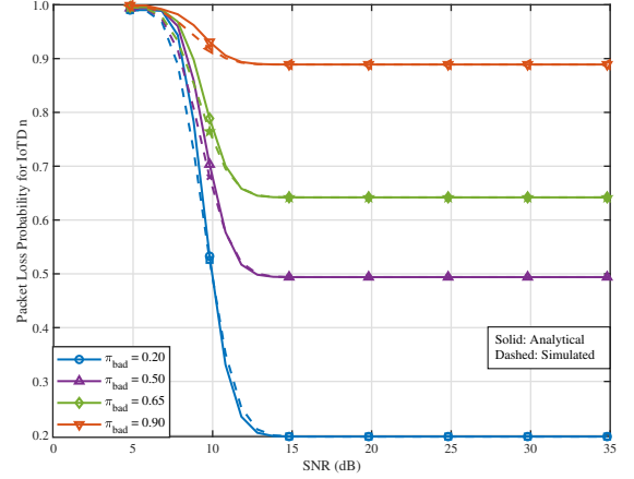
Figure 6. Simulated numerical vs. analytical approximation for various transition probabilities, ( K_1 = K_2 = 10 ).
