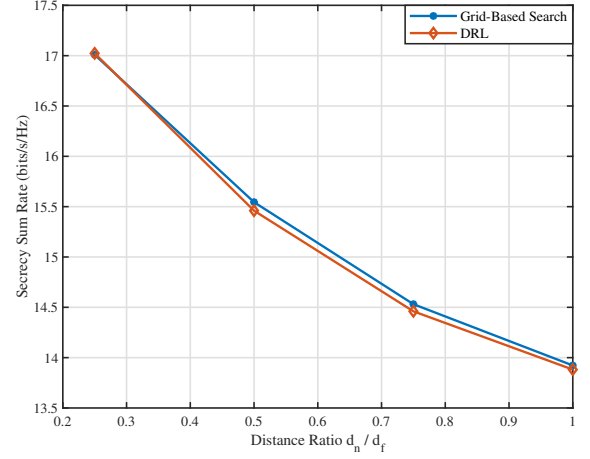
Figure 14. R_s for DRL versus GBS. d_t=2 , d_n \in [1, 4] m, d_f=4 m, d_e=6 m.
