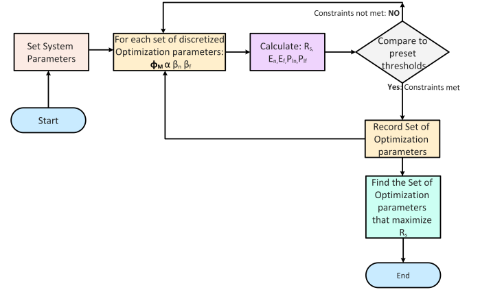
Figure 12. Flow chart of the grid-based methodology.
