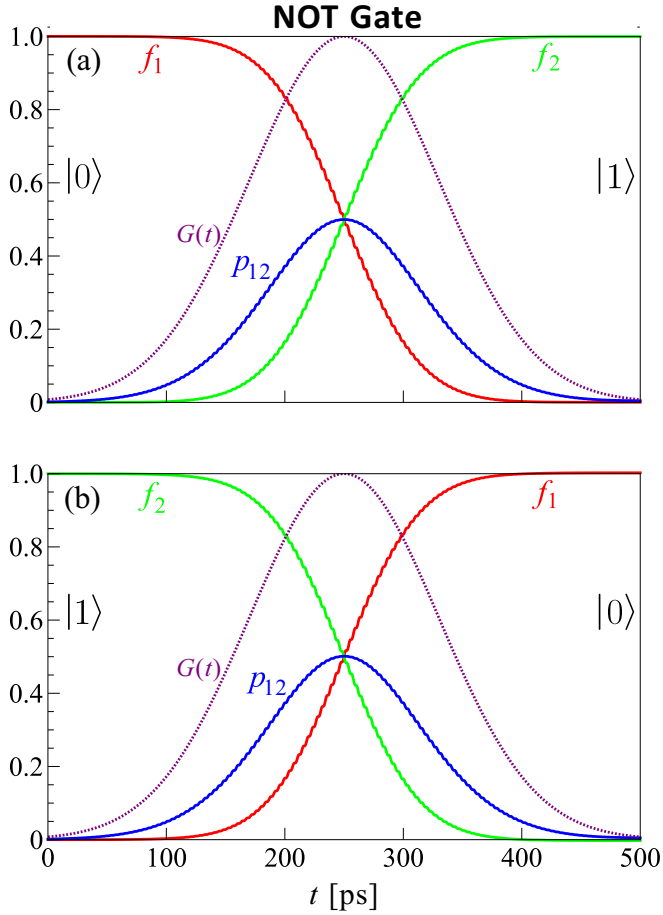
FIG. 6. Simulation of the implementation of a NOT gate in the QSHI-based ASQ. A magnetic \delta impurity characterized by transmission coefficient T_\delta = 0.8 is located at position x_0 = L/4 inside the JJ weak link. The length parameter is \lambda = 2 , and the superconducting phase difference is \phi = \pi/2 .
