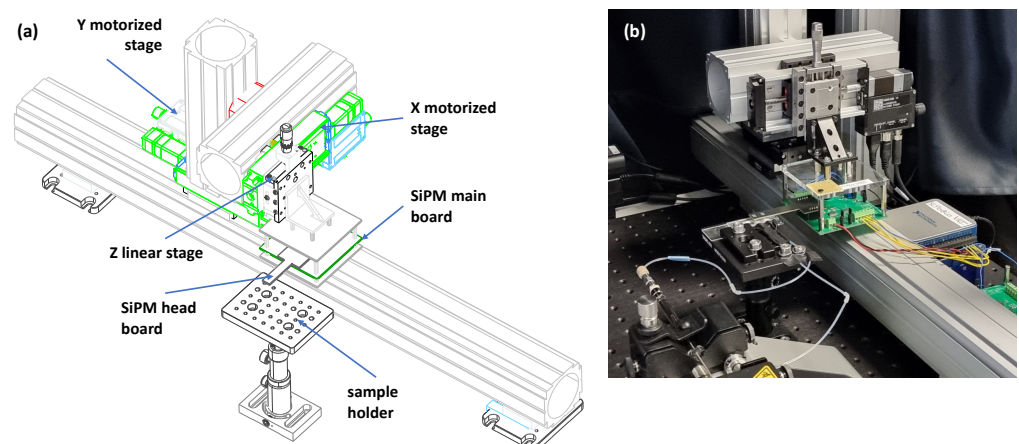
Figure 1. Mechanical layout of the device. (a) Sketch of the biosensors: movement mechanism, sample positioning and board. (b) Picture of the complete device.
