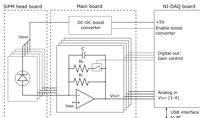
Figure 4. Readout system schematic diagram, see text for details.
