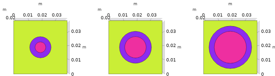
Fig. 4. From left to right, meta-core unit cells with \frac{r}{d} = 0.2 , \frac{r}{d} = 0.3 and \frac{r}{d} = 0.4 .
