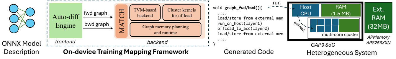
Figure 1: Automatic deployment of DNN training on an ultra-low power system composed of a heterogeneous processor and an external RAM memory.
