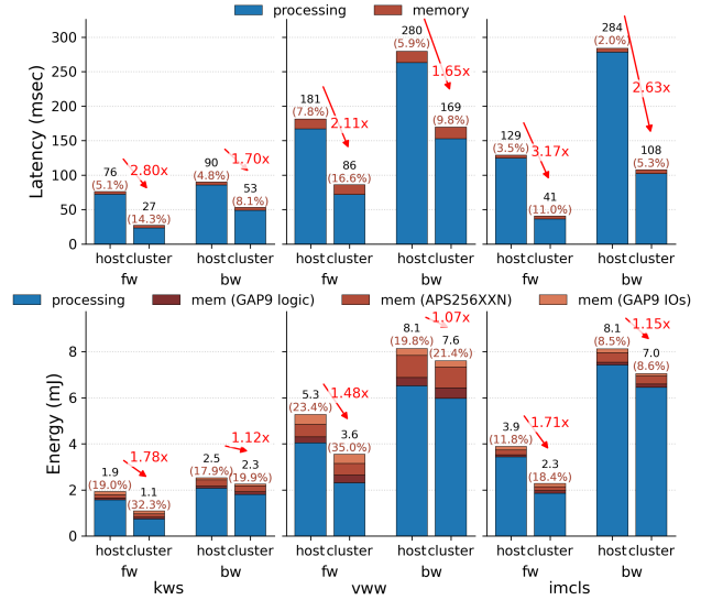
Figure 3: Latency and energy measurements when running ODL on the host CPU ( host ) or on the cluster accelerator. Processing and memory costs are shown separately for the fw and bw tasks. The total values and the memory usage ratio (in parentheses) are indicated at the top of each bar.
