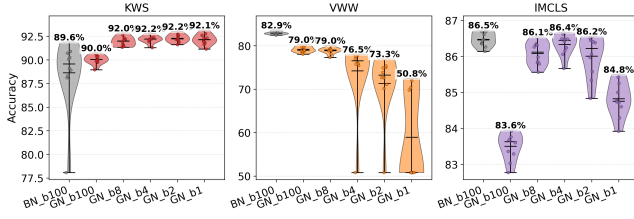
Figure 2: Accuracy with respect to the batch size ( b ). BN and GN stand for BatchNorm and GroupNorm, respectively. The box plot statistics are based on 10 training runs. The mean values are reported above the boxes.
