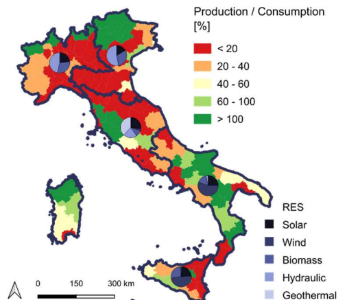
Fig. 2 Ratio between actual production by RES and annual consumption ( P_a/C ).
