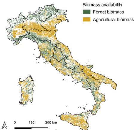
Fig. 3 Spatial distribution of annual available biomass
