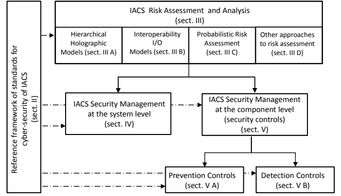
Fig. 2. Basic building blocks for IACS security
