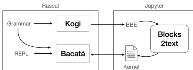
Figure 3. Noteblocks’s architecture
