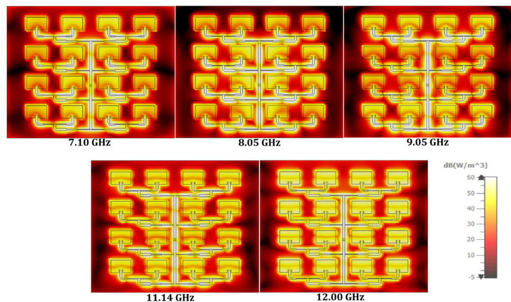
Figure 3. Computed spatial power loss density ( Q_{em} ) distributions across the array aperture and lossy substrate for all five operating frequencies, illustrating the highlighted frequency-dependent thermal excitation nodes.
