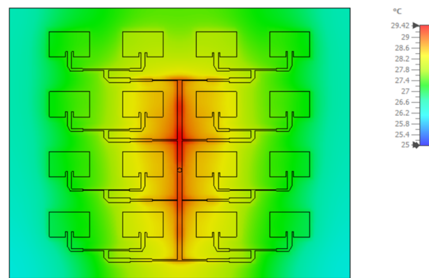
Figure 8. Simulated temperature distribution on the surface of the antenna after 50 s of excitation at 12 GHz.
