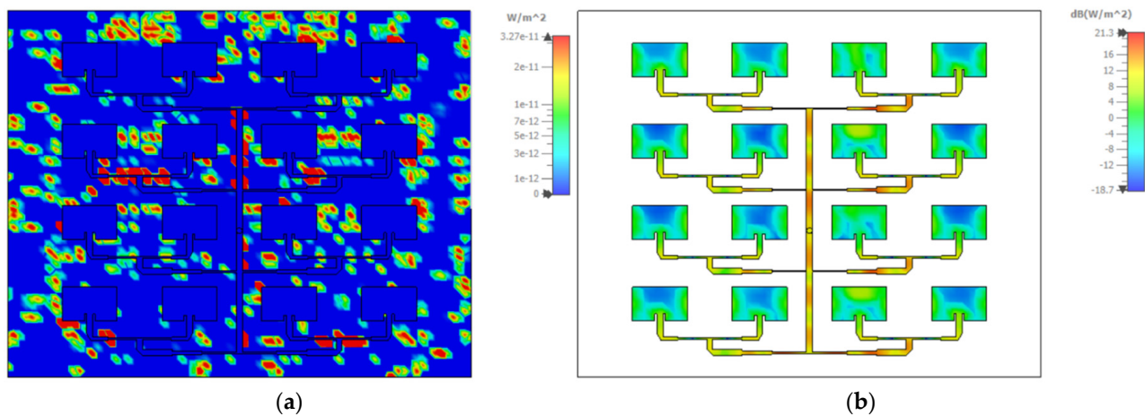
Figure 4. Numerical thermal simulation results after 50 s of MW excitation at 12 GHz: (a) internal heat flow density distribution within the dielectric substrate; (b) surface thermal energy losses across the conductor traces.
