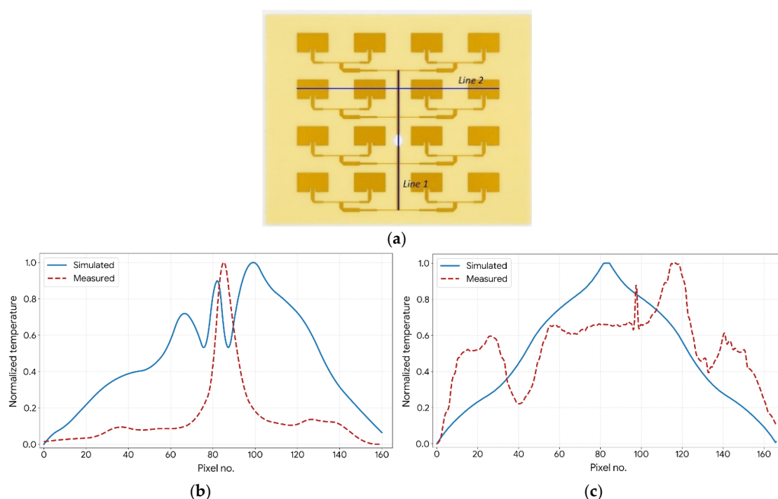
Figure 9. (a) The defined longitudinal (L1) and transversal (L2) axes across the active area; (b) Simulated versus measured temperature distribution along L1 line; (c) Simulated versus measured temperature distribution along L2 line—after 50 s of excitation at 12 GHz.
