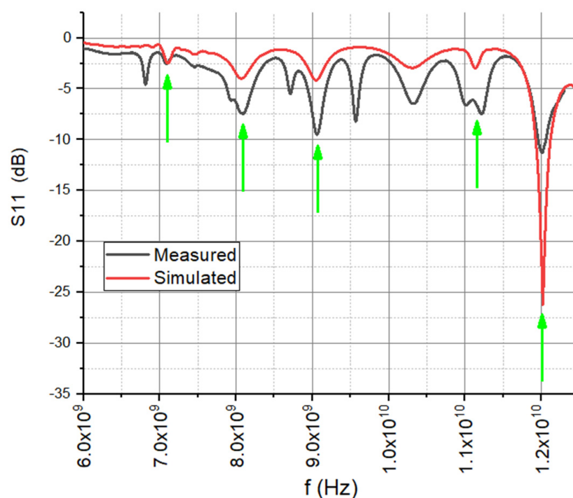
Figure 1. Reflection coefficient (S11) frequency response of the 4 \times 4 patch array, comparing CST full-wave numerical simulation (red curve) with experimental vector network analyzer measurements (black curve). Green arrows indicate the five target operating frequencies evaluated in this study.
