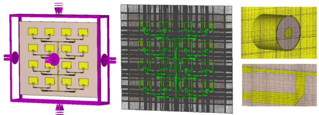
Figure 2. Numerical computational domain and discretization setup in CST Studio Suite: 3D CAD model of the 4 \times 4 array, open PML boundary conditions, localized hexahedral mesh refinement along trace edges and 50 \Omega waveguide port model.
