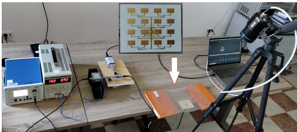
Figure 6. Experimental testbed layout for non-invasive transient IR thermography characterization, showing the continuous-wave (CW) microwave signal delivery chain, the 4 \times 4 patch array positioned beneath the ITO/PET transducer thin film and the Teledyne FLIR A700 IR camera.
