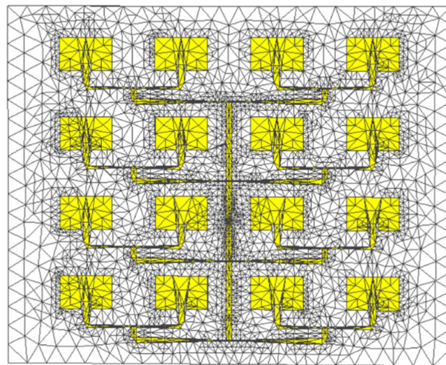
Figure 5. Finite-element thermal mesh discretization across the array geometry, highlighting local mesh refinement and continuum interface matching between the 35 \mu\text{m} thin copper metallization layer and the Rogers RO4350B substrate.
