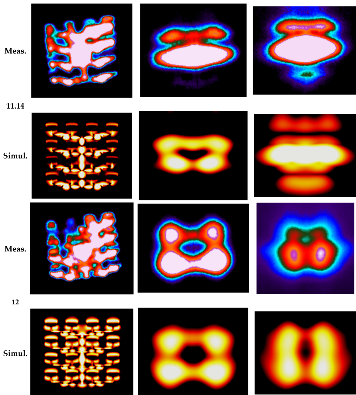
Figure 7. Qualitative and quantitative spatial pattern validation: comparison between calibrated experimental LWIR thermograms (top rows) and full-wave simulated power loss density distributions (bottom rows) across five excitation frequencies (7.10, 8.05, 9.05, 11.14, and 12.00 GHz) at three near-field evaluation planes situated at 1 mm, 16 mm, and 29 mm respectively).
