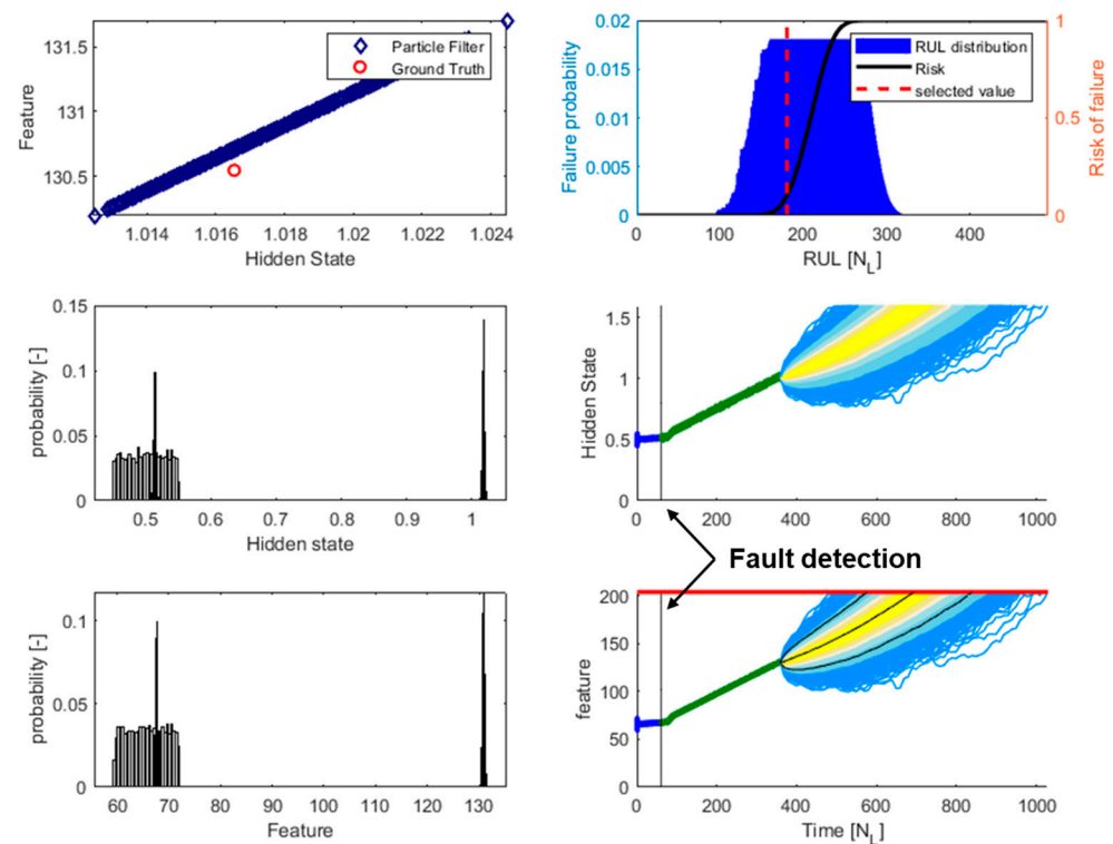
Figure 15. Prognostic performance against simulated dataset ( N_p = 5000 ). The feature values are expressed in radians.
