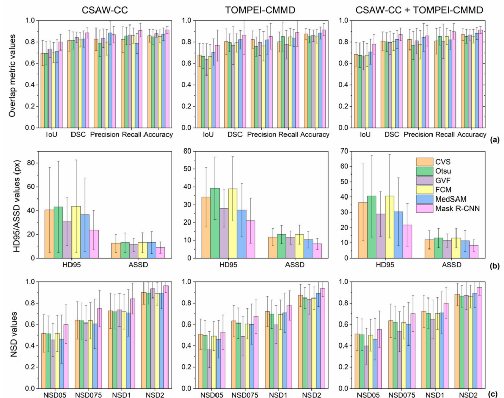
Figure 7. Application of Mask R-CNN model and other segmentation methods (CVS, Otsu thresholding, GVF active contour, FCM and MedSAM) to a set of 155 real mammograms; the predicted masks are compared to the annotated masks provided by CSAW-CC and TOMPEI-CMMD, used as reference. Evaluation of segmentation performance by means of (a) overlap-based metrics (IoU, DSC, Precision, Recall and Accuracy), distance-based metrics (b) HD95 and ASSD, and (c) NSD with \tau equal to 0.5 mm, 0.75 mm, 1 mm and 2 mm. From left to right, the graphs report the results for the images from CSAW-CC, TOMPEI-CMMD, and the two combined datasets, respectively.
