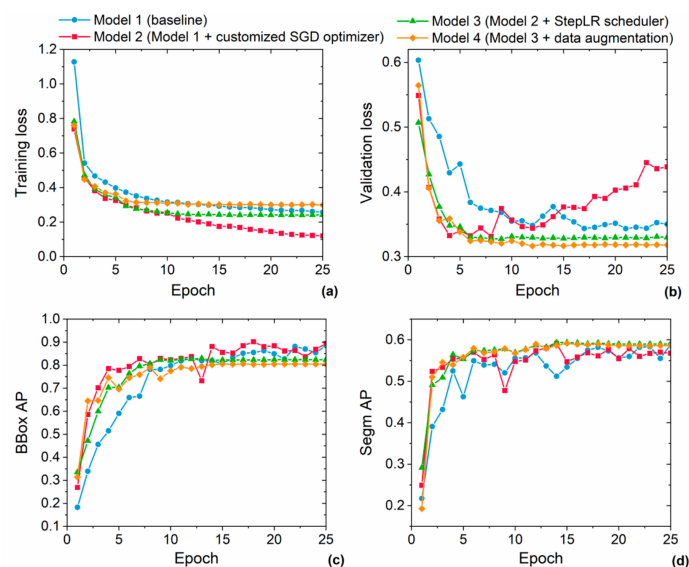
Figure 2. Comparison of Mask R-CNN model configurations along the training/validation pipeline, in terms of (a) training loss, (b) validation loss, (c) bounding box average precision (BBox AP) and (d) segmentation average precision (Segm AP). For BBox AP and Segm AP values, we consider IoU = 0.5:0.95.
