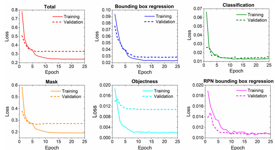
Figure 3. Loss components vs. epoch of the Mask R-CNN model configuration with StepLR scheduler (Model 3), during training and validation phases. The panels contain (from left to right, top to bottom) the total, bounding box regression, classification, mask, objectness and RPN bounding box regression losses. The solid lines represent the training curves, whereas the dotted lines indicate the corresponding validation curves.
