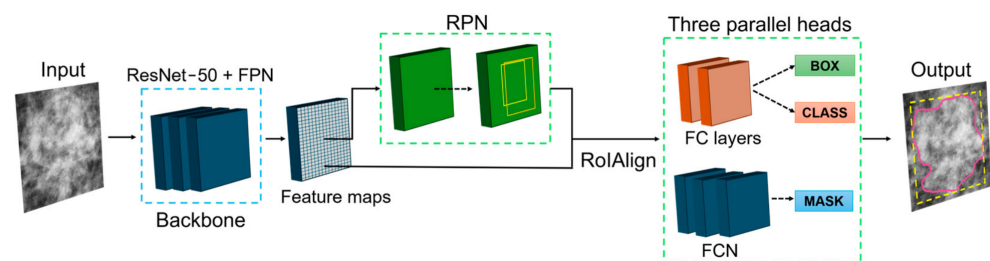
Figure 1. Schematics of the deep learning segmentation model based on Mask R-CNN used for the contouring of breast lesion masses.
