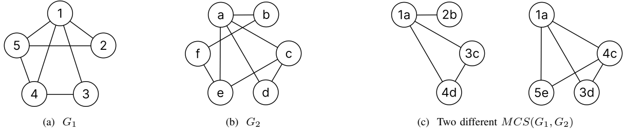
Fig. 1. Given the graphs G_1 and G_2 represented in Figures (a) and (b), respectively, Figure (c) reports two different admissible MCSs. Labels are shown only to help identify the vertices, as the graphs are not to be considered labeled.
