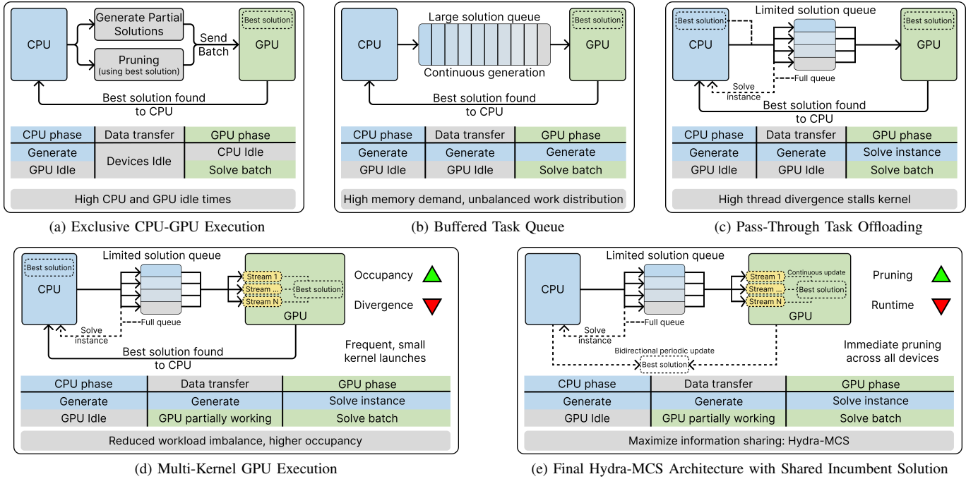
Fig. 4. Successive Hydra-MCS design variants, i.e., logical evolution of CPU-GPU interaction strategies leading to the final architecture of Hydra-MCS. The diagrams reflect the sequential descriptions provided in the text, with accompanying notes at the bottom highlighting the salient characteristics of each strategy.
