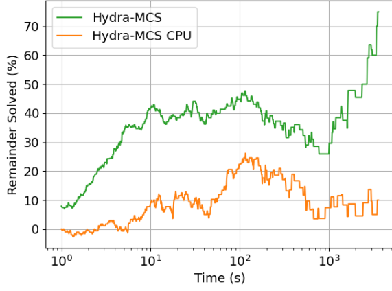
Fig. 8. Percentage of instances deemed intractable by the McSplit baseline that were successfully solved by competing approaches.
