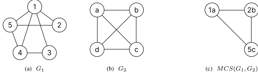
Fig. 2. The figure shows two undirected, unlabeled graphs, G_1 and G_2 , along with a common subgraph identified by the McSplit algorithm. Vertex identifiers, i.e., \{1, 2, 3, 4, 5\} for G_1 and \{a, b, c, d\} for G_2 , are used solely for unique identification and do not represent vertex labels.
