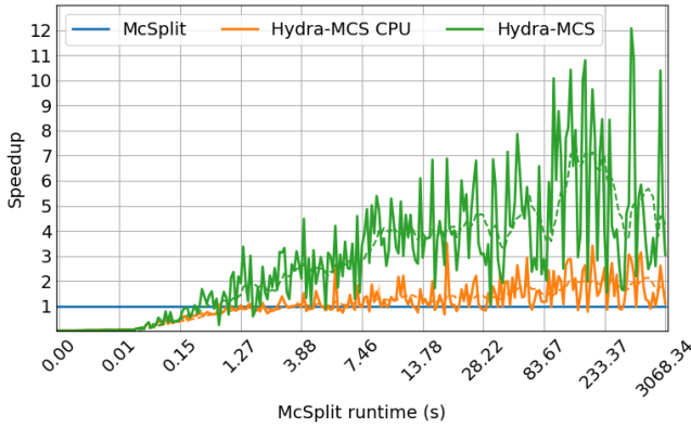
Fig. 5. Speedup of our CPU-only and CPU-GPU approaches compared to the original McSplit procedure (the fastest algorithm we tested for finding maximal solutions to the problems).
