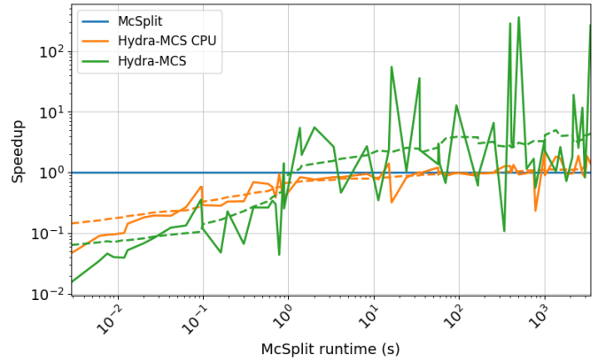
Fig. 10. Speedup of CPU-only and hybrid Hydra-MCS over multithreaded McSplit on the 66 solved graph pairs containing from 60 to 100 nodes. Solid curves show per-instance speedups; dashed curves show moving geometric means.
